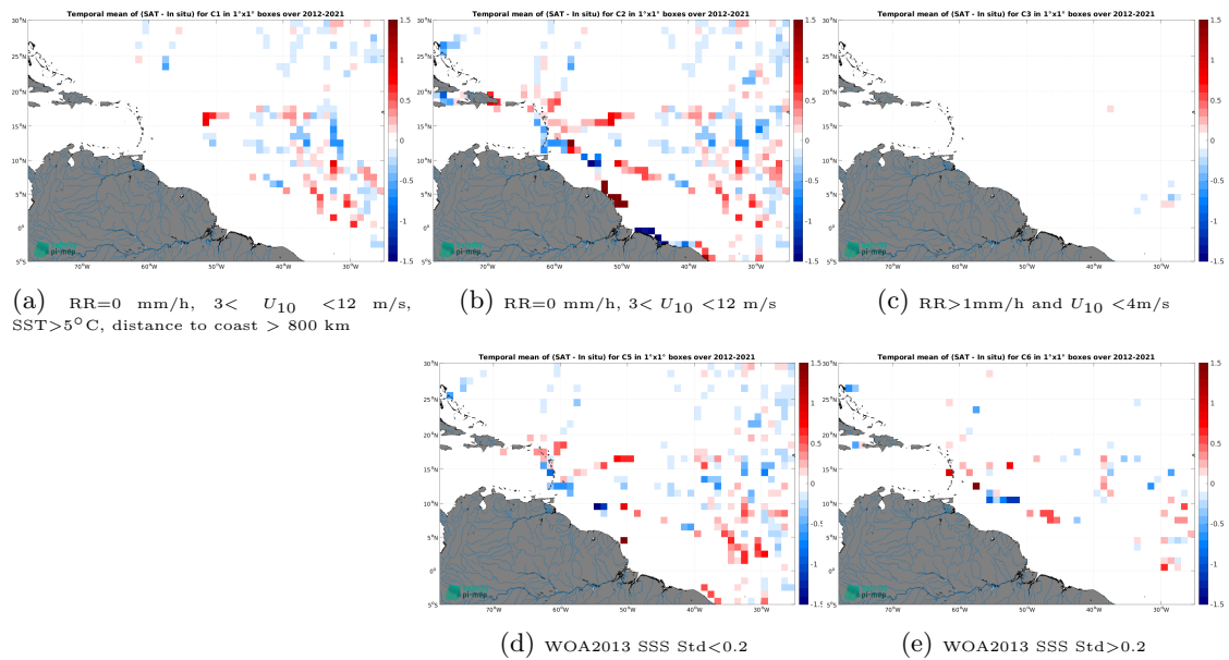
Figure 14: Temporal mean gridded over spatial boxes of size 1^\circ \times 1^\circ of \Delta SSS (SMOS SSS L4 v1 - Daily (CMEMS-CNR) - TSG (GOSUD-Sailing-ship)) for 5 different subdatasets corresponding to:RR=0 mm/h, 3 < U_{10} < 12 m/s, SST >5^\circ\text{C} , distance to coast > 800 km (a), RR=0 mm/h, 3 < U_{10} < 12 m/s (b), RR >1 mm/h and U_{10} < 4 m/s (c), WOA2013 SSS Std <0.2 (d), WOA2013 SSS Std >0.2 (e).
