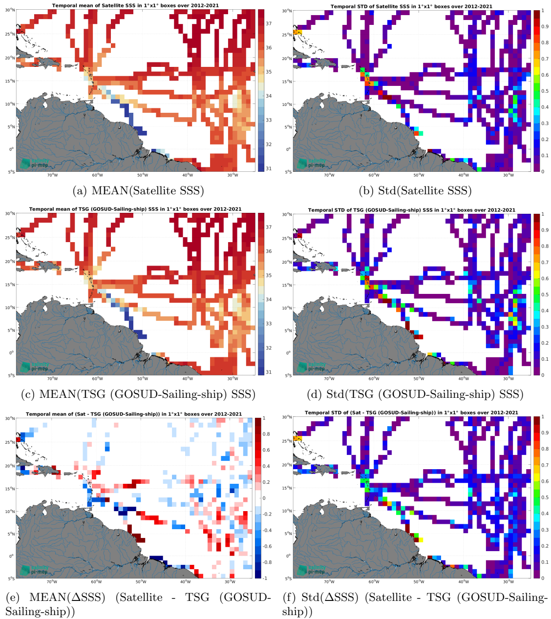
Figure 7: Temporal mean (left) and Std (right) of SSS from SMOS SSS L4 v1 - Daily (CMEMS-CNR) (top), TSG (GOSUD-Sailing-ship) (middle), and of \Delta SSS (Satellite - TSG (GOSUD-Sailing-ship)). Only match-up pairs are used to generate these maps.
