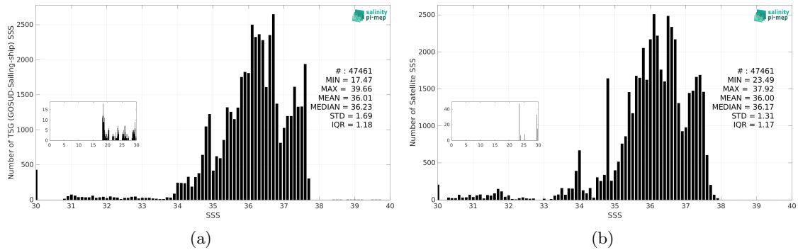
Figure 3: Histograms of SSS from TSG (GOSUD-Sailing-ship) (a) and SMOS SSS L4 v1 - Daily (CMEMS-CNR) (b) considering all match-up pairs per bins of 0.1 over the Amazon and Orinoco river plumes Pi-MEP region and for the full satellite product period.
