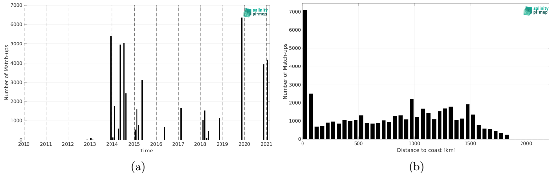
Figure 2: Number of match-ups between TSG (GOSUD-Sailing-ship) and SMOS SSS L4 v1 - Daily (CMEMS-CNR) SSS as a function of time (a) and as function of the distance to coast (b) over the Amazon and Orinoco river plumes Pi-MEP region and for the full satellite product period.
