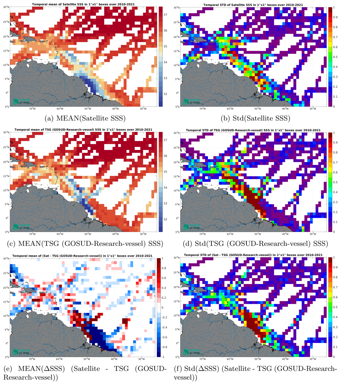
Figure 7: Temporal mean (left) and Std (right) of SSS from SMOS SSS L4 v1 - Daily (CMEMS-CNR) (top), TSG (GOSUD-Research-vessel) (middle), and of \Delta SSS (Satellite - TSG (GOSUD-Research-vessel)). Only match-up pairs are used to generate these maps.
