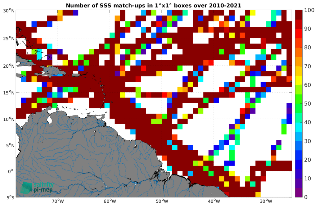
Figure 5: Number of SSS match-ups between TSG (GOSUD-Research-vessel) SSS and the SMOS SSS L4 v1 - Daily (CMEMS-CNR) SSS product for the Amazon and Orinoco river plumes Pi-MEP region over 1^\circ \times 1^\circ boxes and for the full satellite product period.
