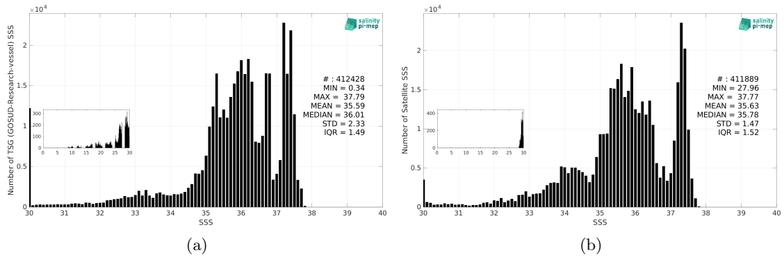
Figure 3: Histograms of SSS from TSG (GOSUD-Research-vessel) (a) and SMOS SSS L4 v1 - Daily (CMEMS-CNR) (b) considering all match-up pairs per bins of 0.1 over the Amazon and Orinoco river plumes Pi-MEP region and for the full satellite product period.
