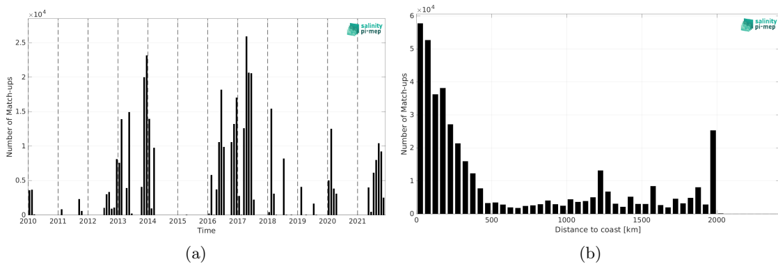
Figure 2: Number of match-ups between TSG (GOSUD-Research-vessel) and SMOS SSS L4 v1 - Daily (CMEMS-CNR) SSS as a function of time (a) and as function of the distance to coast (b) over the Amazon and Orinoco river plumes Pi-MEP region and for the full satellite product period.
