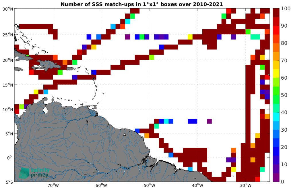
Figure 5: Number of SSS match-ups between TSG (CSIC-UTM) SSS and the SMOS SSS L4 v1 - Daily (CMEMS-CNR) SSS product for the Amazon and Orinoco river plumes Pi-MEP region over 1^{\circ} \times 1^{\circ} boxes and for the full satellite product period.
