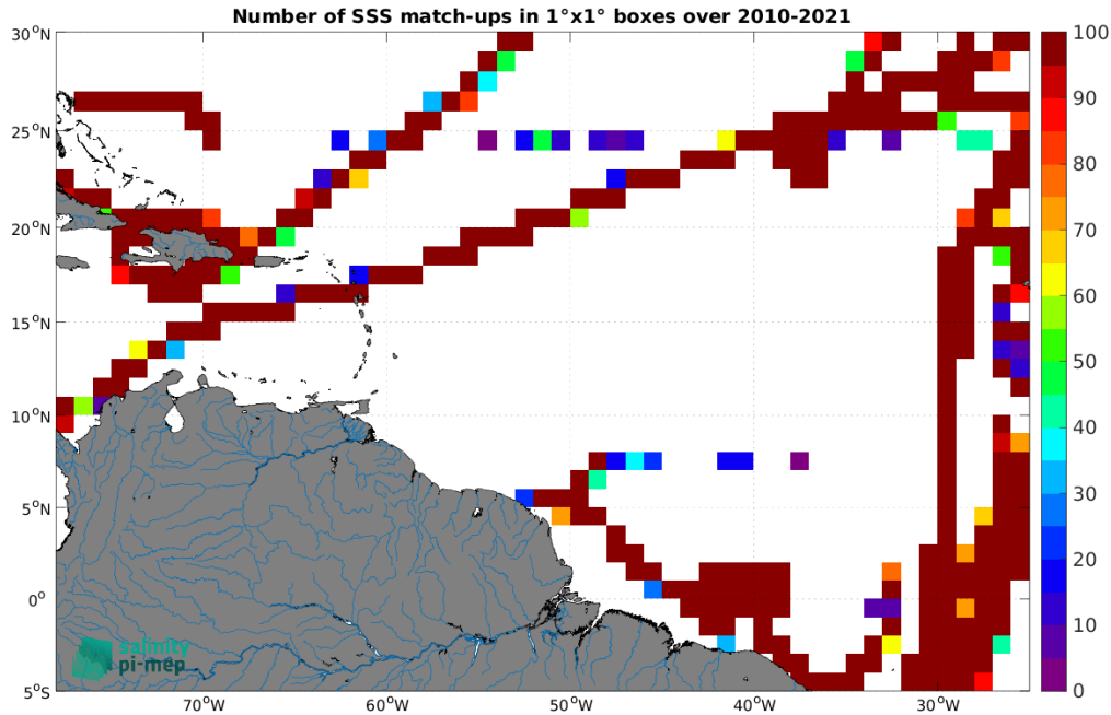
Figure 5: Number of SSS match-ups between TSG (CSIC-UTM) SSS and the SMOS SSS L4 v1 - Daily (CMEMS-CNR) SSS product for the Amazon and Orinoco river plumes Pi-MEP region over 1^\circ \times 1^\circ boxes and for the full satellite product period.
