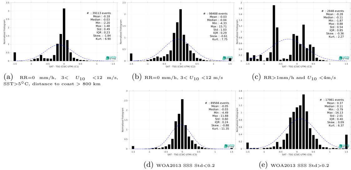
Figure 15: Normalized histogram of \Delta SSS (SMOS SSS L4 v1 - Daily (CMEMS-CNR) - TSG (CSIC-UTM)) for 5 different subdatasets corresponding to: RR=0 mm/h, 3 < U_{10} < 12 m/s, SST>5°C, distance to coast > 800 km (a), RR=0 mm/h, 3 < U_{10} < 12 m/s (b), RR>1mm/h and U_{10} < 4 m/s (c), WOA2013 SSS Std<0.2 (d), WOA2013 SSS Std>0.2 (e).
