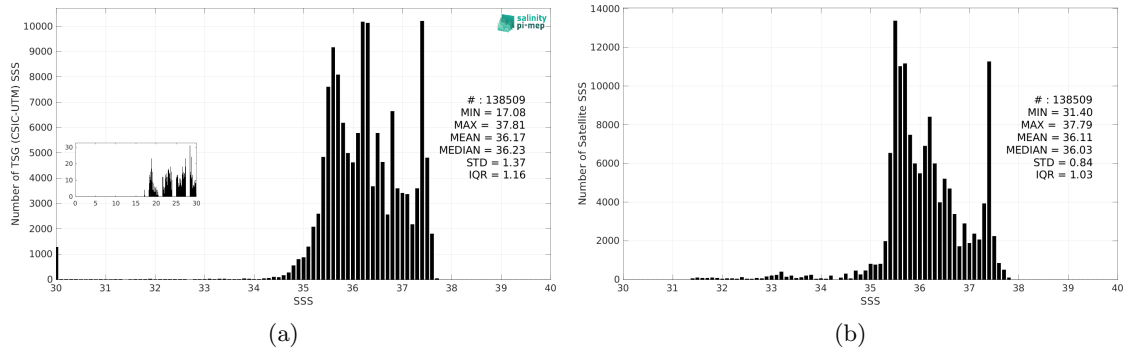
Figure 3: Histograms of SSS from TSG (CSIC-UTM) (a) and SMOS SSS L4 v1 - Daily (CMEMS-CNR) (b) considering all match-up pairs per bins of 0.1 over the Amazon and Orinoco river plumes Pi-MEP region and for the full satellite product period.
