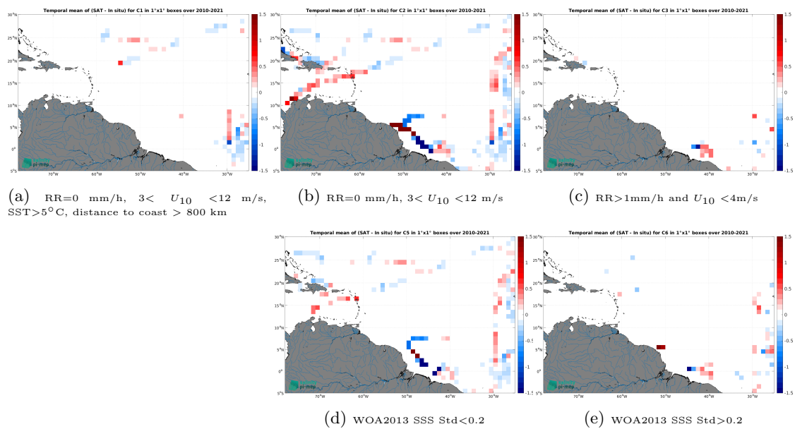
Figure 14: Temporal mean gridded over spatial boxes of size 1^\circ \times 1^\circ of \Delta SSS (SMOS SSS L4 v1 - Daily (CMEMS-CNR) - TSG (CSIC-UTM)) for 5 different subdatasets corresponding to:RR=0 mm/h, 3 < U_{10} < 12 m/s, SST >5^\circ\text{C} , distance to coast > 800 km (a), RR=0 mm/h, 3 < U_{10} < 12 m/s (b), RR >1 mm/h and U_{10} < 4 m/s (c), WOA2013 SSS Std <0.2 (d), WOA2013 SSS Std >0.2 (e).
