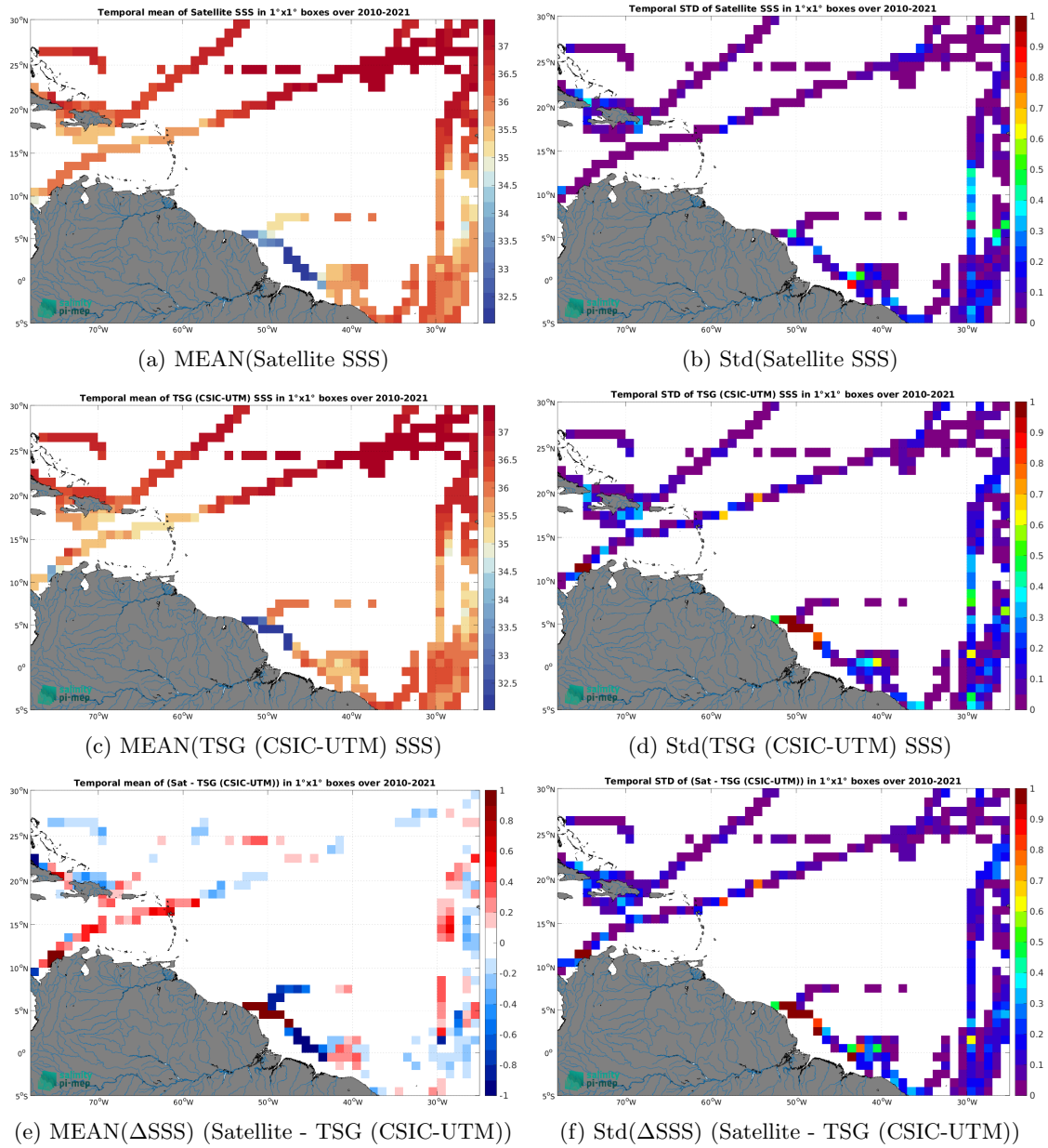
Figure 7: Temporal mean (left) and Std (right) of SSS from SMOS SSS L4 v1 - Daily (CMEMS-CNR) (top), TSG (CSIC-UTM) (middle), and of \Delta SSS (Satellite - TSG (CSIC-UTM)). Only match-up pairs are used to generate these maps.
