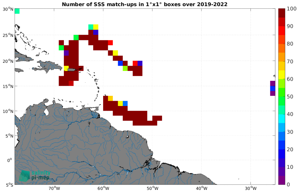
Figure 5: Number of SSS match-ups between Saildrone SSS and the SMOS SSS L4 v1 - Daily (CMEMS-CNR) SSS product for the Amazon and Orinoco river plumes Pi-MEP region over 1°x1° boxes and for the full satellite product period.
