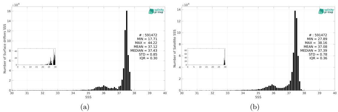
Figure 3: Histograms of SSS from Surface drifters (a) and SMOS SSS L4 v1 - Daily (CMEMS-CNR) (b) considering all match-up pairs per bins of 0.1 over the Amazon and Orinoco river plumes Pi-MEP region and for the full satellite product period.
