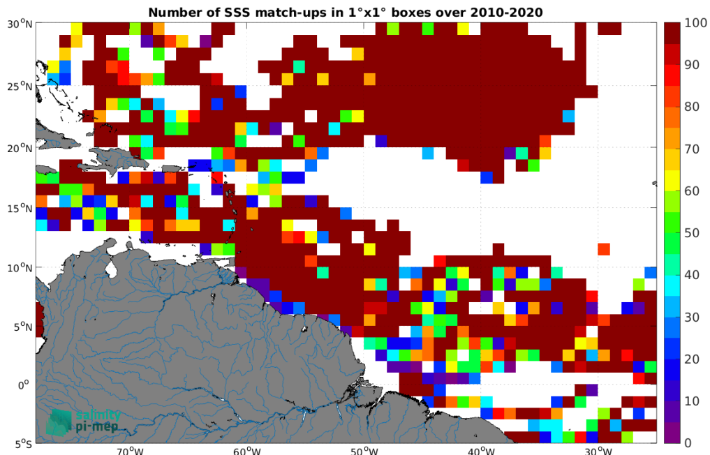
Figure 4: Number of SSS match-ups between Surface drifters SSS and the SMOS SSS L4 v1 - Daily (CMEMS-CNR) SSS product for the Amazon and Orinoco river plumes Pi-MEP region over 1^\circ \times 1^\circ boxes and for the full satellite product period.
