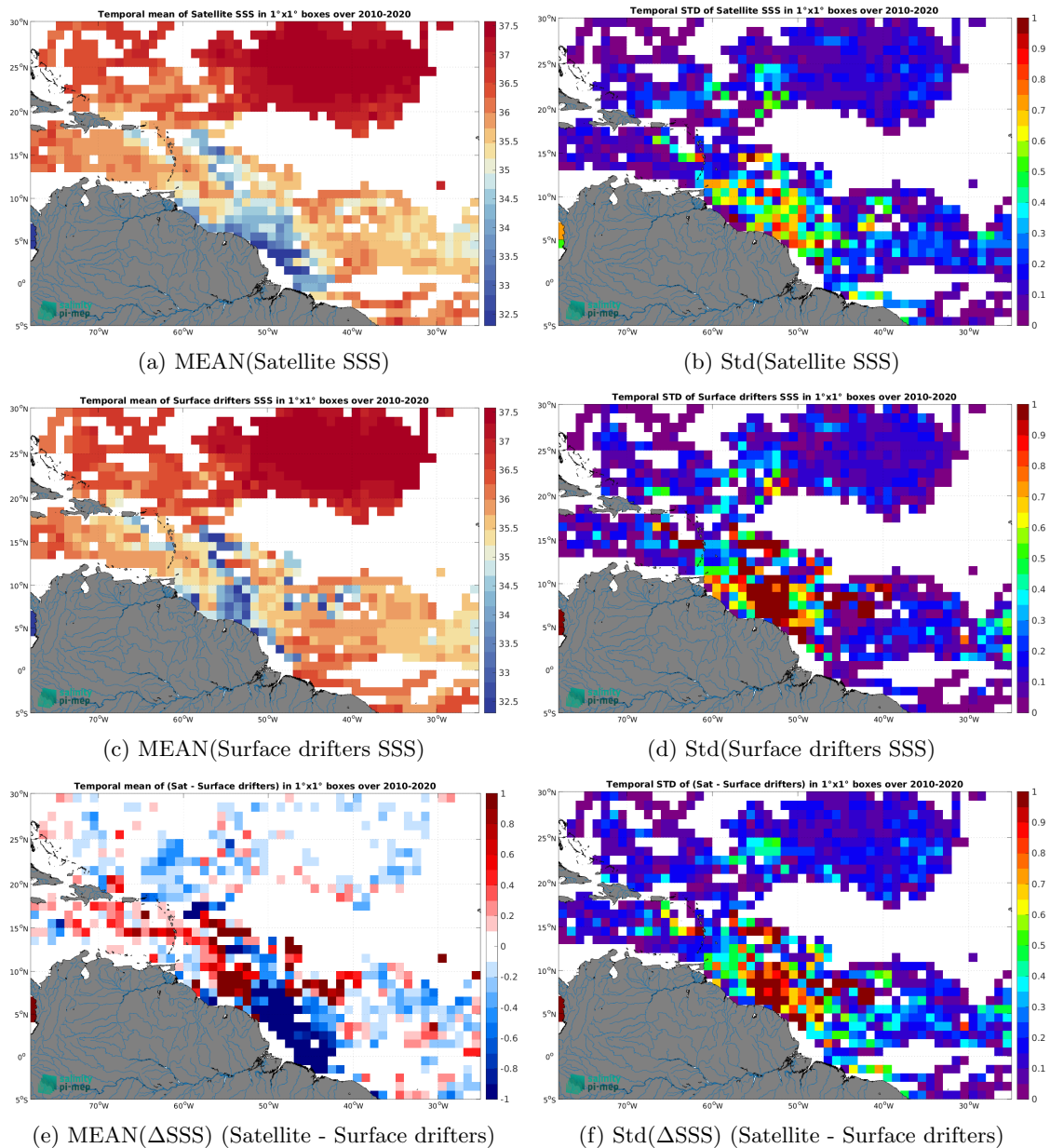
Figure 6: Temporal mean (left) and Std (right) of SSS from SMOS SSS L4 v1 - Daily (CMEMS-CNR) (top), Surface drifters (middle), and of \Delta SSS (Satellite - Surface drifters). Only match-up pairs are used to generate these maps.
