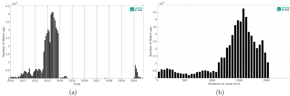
Figure 2: Number of match-ups between Surface drifters and SMOS SSS L4 v1 - Daily (CMEMS-CNR) SSS as a function of time (a) and as function of the distance to coast (b) over the Amazon and Orinoco river plumes Pi-MEP region and for the full satellite product period.
