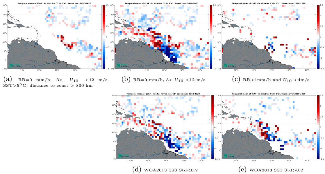
Figure 13: Temporal mean gridded over spatial boxes of size 1^\circ \times 1^\circ of \Delta\text{SSS} (SMOS SSS L4 v1 - Daily (CMEMS-CNR) - Surface drifters) for 5 different subdatasets corresponding to:RR=0 mm/h, 3 < U_{10} < 12 m/s, SST >5^\circ\text{C} , distance to coast > 800 km (a), RR=0 mm/h, 3 < U_{10} < 12 m/s (b), RR >1 mm/h and U_{10} < 4 m/s (c), WOA2013 SSS Std <0.2 (d), WOA2013 SSS Std >0.2 (e).
