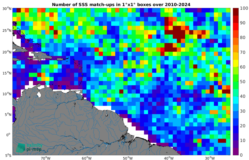
Figure 5: Number of SSS match-ups between Argo SSS and the SMOS SSS L4 v1 - Daily (CMEMS-CNR) SSS product for the Amazon and Orinoco river plumes Pi-MEP region over 1^\circ \times 1^\circ boxes and for the full satellite product period.
