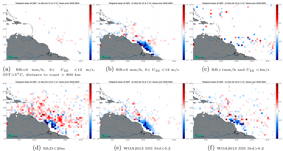
Figure 14: Temporal mean gridded over spatial boxes of size 1^\circ \times 1^\circ of \Delta SSS (SMOS SSS L4 v1 - Daily (CMEMS-CNR) - Argo) for 6 different subdatasets corresponding to:RR=0 mm/h, 3 < U_{10} < 12 m/s, SST >5^\circ C, distance to coast > 800 km (a), RR=0 mm/h, 3 < U_{10} < 12 m/s (b), RR >1 mm/h and U_{10} < 4 m/s (c),MLD <20 m (d),WOA2013 SSS Std <0.2 (e),WOA2013 SSS Std >0.2 (f).
