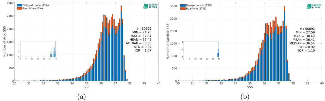
Figure 3: Histograms of SSS from Argo (a) and SMOS SSS L4 v1 - Daily (CMEMS-CNR) (b) considering all match-up pairs per bins of 0.1 over the Amazon and Orinoco river plumes Pi-MEP region and for the full satellite product period.
