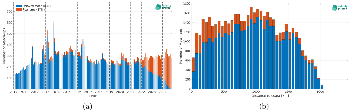
Figure 2: Number of match-ups between Argo and SMOS SSS L4 v1 - Daily (CMEMS-CNR) SSS as a function of time (a) and as function of the distance to coast (b) over the Amazon and Orinoco river plumes Pi-MEP region and for the full satellite product period.
