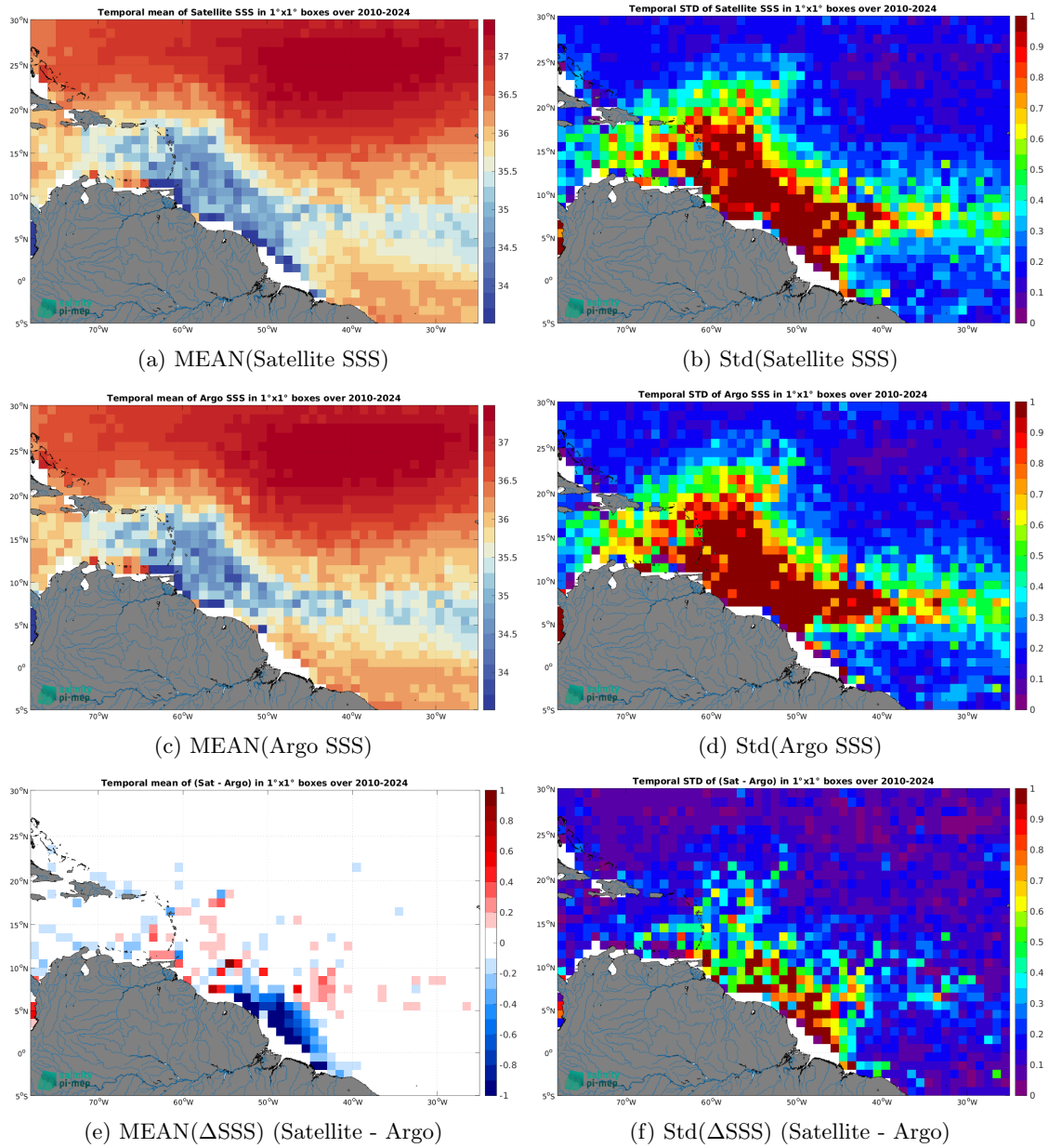
Figure 7: Temporal mean (left) and Std (right) of SSS from SMOS SSS L4 v1 - Daily (CMEMS-CNR) (top), Argo (middle), and of \Delta SSS (Satellite - Argo). Only match-up pairs are used to generate these maps.
