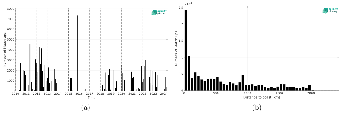
Figure 2: Number of match-ups between TSG (SAMOS) and SMOS SSS L4 OI v346 - Weekly (CMEMS-CATDS-LOPS) SSS as a function of time (a) and as function of the distance to coast (b) over the Amazon and Orinoco river plumes Pi-MEP region and for the full satellite product period.
