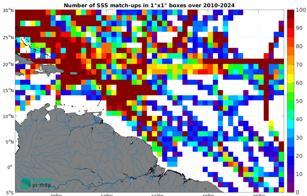
Figure 5: Number of SSS match-ups between TSG (SAMOS) SSS and the SMOS SSS L4 OI v346 - Weekly (CMEMS-CATDS-LOPS) SSS product for the Amazon and Orinoco river plumes Pi-MEP region over 1^\circ \times 1^\circ boxes and for the full satellite product period.
