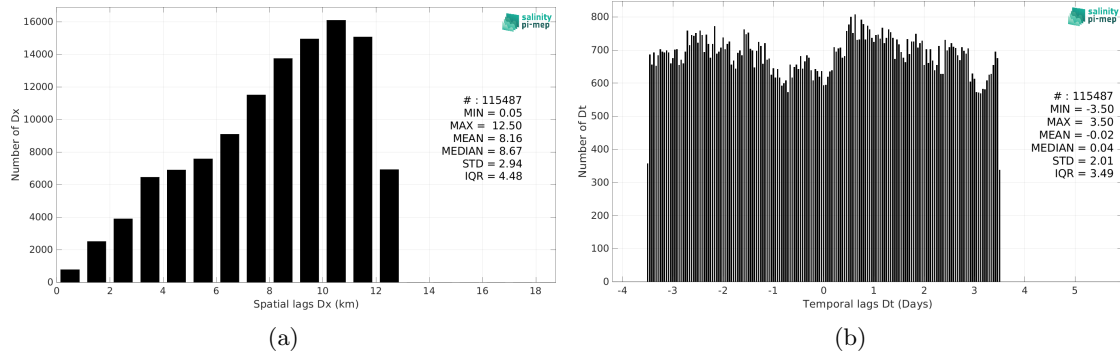
Figure 6: Histograms of the spatial (a) and temporal (b) lags between the location/time of the TSG (SAMOS) measurement and the date of the corresponding SMOS SSS L4 OI v346 - Weekly (CMEMS-CATDS-LOPS) SSS pixel.
