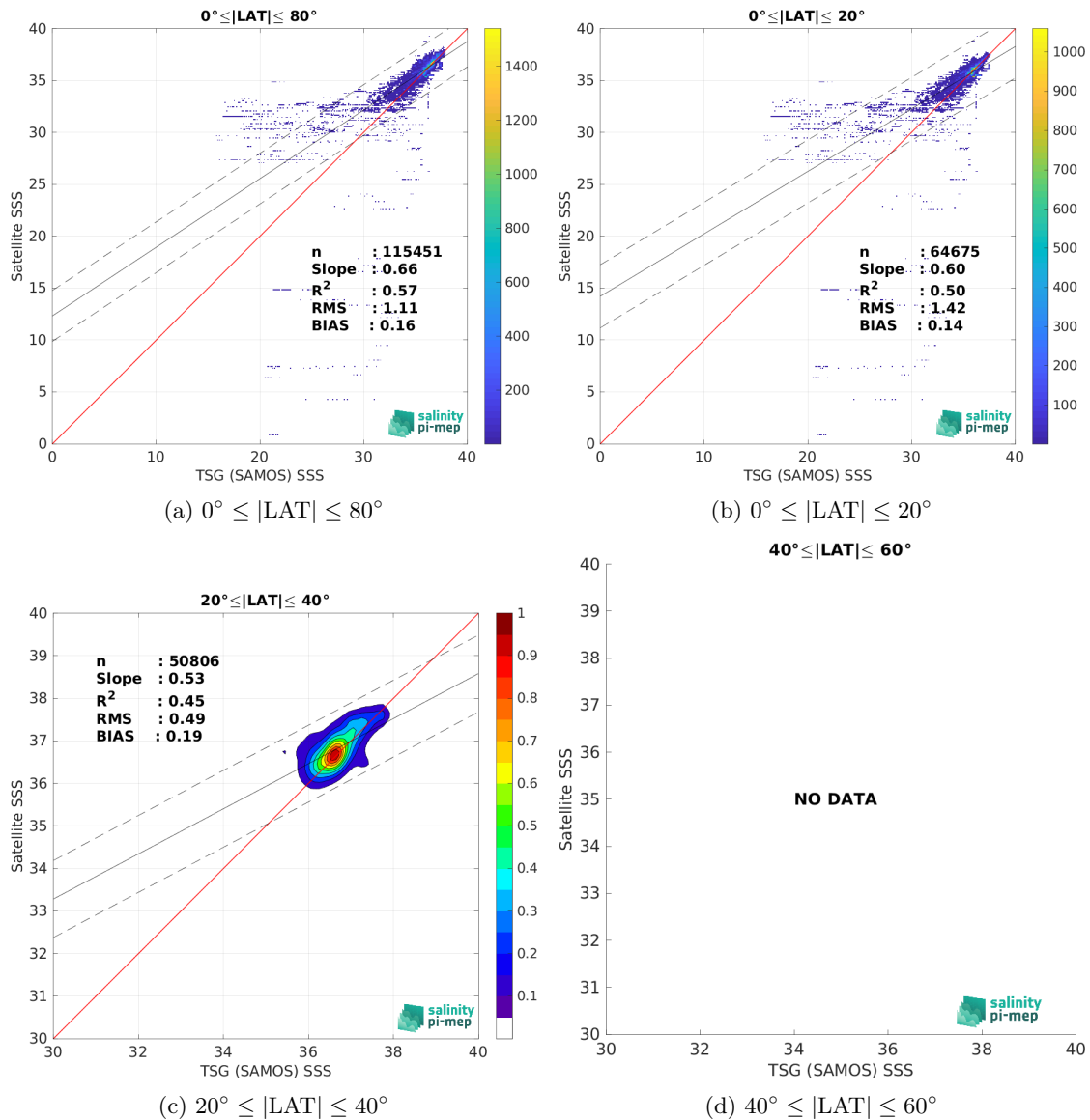
Figure 10: Contour maps of the concentration of SMOS SSS L4 OI v346 - Weekly (CMEMS-CATDS-LOPS) SSS (y-axis) versus TSG (SAMOS) SSS (x-axis) at match-up pairs for different latitude bands. For each plot, the red line shows x=y . The black thin and dashed lines indicate a linear fit through the data cloud and the \pm 95\% confidence levels, respectively. The number match-up pairs n , the slope and R^2 coefficient of the linear fit, the root mean square (RMS) and the mean bias between satellite and in situ data are indicated for each latitude band in each plots.
