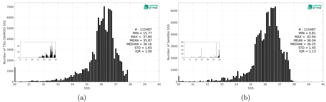
Figure 3: Histograms of SSS from TSG (SAMOS) (a) and SMOS SSS L4 OI v346 - Weekly (CMEMS-CATDS-LOPS) (b) considering all match-up pairs per bins of 0.1 over the Amazon and Orinoco river plumes Pi-MEP region and for the full satellite product period.
