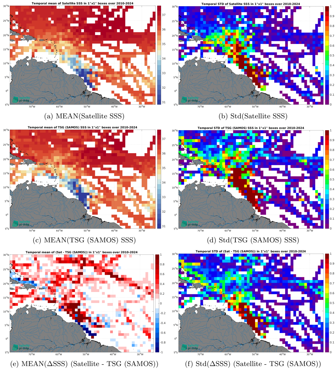
Figure 7: Temporal mean (left) and Std (right) of SSS from SMOS SSS L4 OI v346 - Weekly (CMEMS-CATDS-LOPS) (top), TSG (SAMOS) (middle), and of \Delta SSS (Satellite - TSG (SAMOS)). Only match-up pairs are used to generate these maps.
