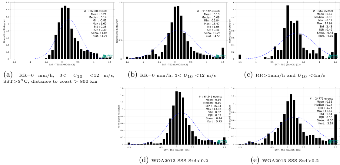
Figure 15: Normalized histogram of \Delta SSS (SMOS SSS L4 OI v346 - Weekly (CMEMS-CATDS-LOPS) - TSG (SAMOS)) for 5 different subdatasets corresponding to: RR=0 mm/h, 3 < U_{10} < 12 m/s, SST>5°C, distance to coast > 800 km (a), RR=0 mm/h, 3 < U_{10} < 12 m/s (b), RR>1mm/h and U_{10} < 4 m/s (c), WOA2013 SSS Std<0.2 (d), WOA2013 SSS Std>0.2 (e).
