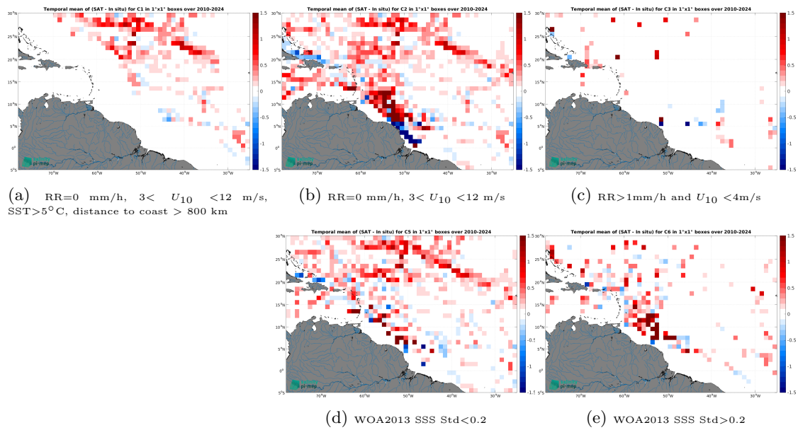
Figure 14: Temporal mean gridded over spatial boxes of size 1^\circ \times 1^\circ of \Delta SSS (SMOS SSS L4 OI v346 - Weekly (CMEMS-CATDS-LOPS) - TSG (SAMOS)) for 5 different subdatasets corresponding to:RR=0 mm/h, 3 < U_{10} < 12 m/s, SST > 5°C, distance to coast > 800 km (a), RR=0 mm/h, 3 < U_{10} < 12 m/s (b), RR > 1mm/h and U_{10} < 4 m/s (c), WOA2013 SSS Std < 0.2 (d), WOA2013 SSS Std > 0.2 (e).
