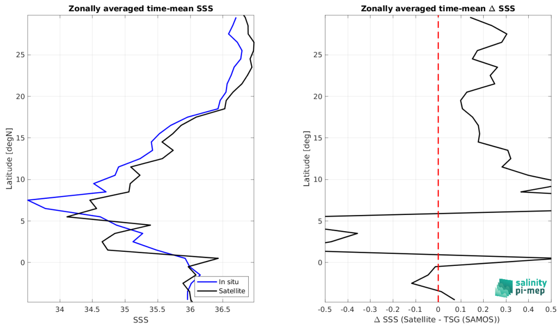
Figure 9: Left panel: Zonal mean SSS from SMOS SSS L4 OI v346 - Weekly (CMEMS-CATDS-LOPS) satellite product (black) and from TSG (SAMOS) (blue). Right panel: Zonal mean of \Delta SSS (Satellite - TSG (SAMOS)) for all the collected Pi-MEP match-up pairs estimated over the full satellite product period.
