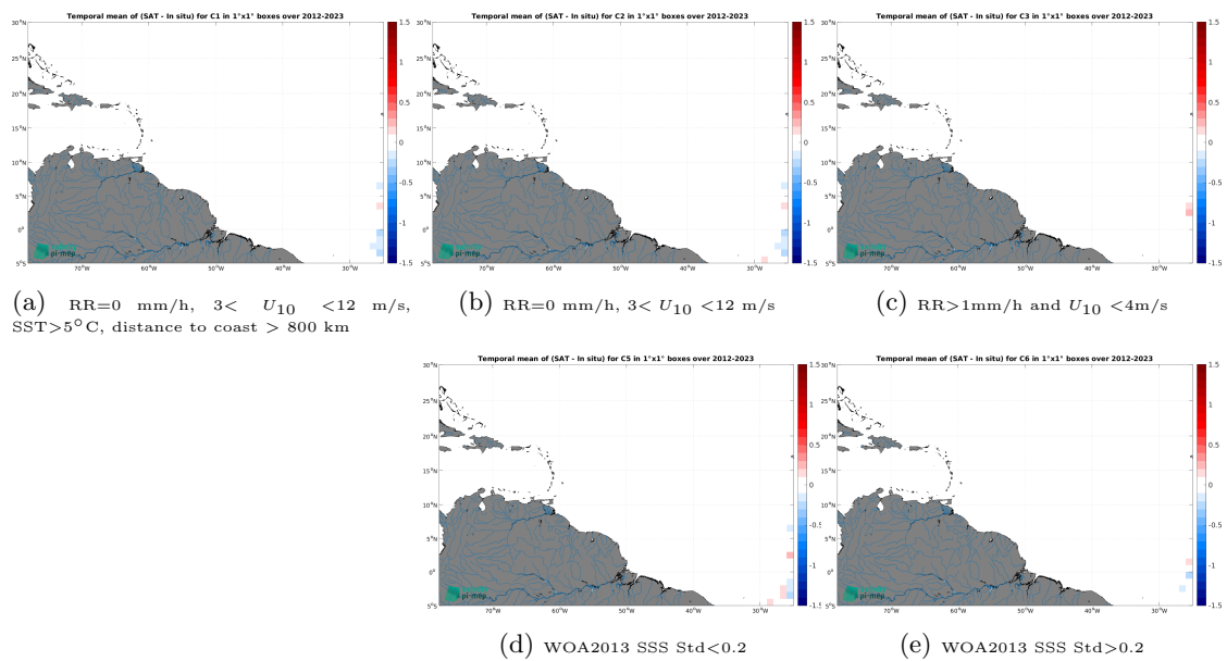
Figure 14: Temporal mean gridded over spatial boxes of size 1^\circ \times 1^\circ of \Delta SSS (SMOS SSS L4 OI v346 - Weekly (CMEMS-CATDS-LOPS) - TSG (Polarstern)) for 5 different subdatasets corresponding to:RR=0 mm/h, 3 < U_{10} < 12 m/s, SST >5^\circ C, distance to coast > 800 km (a), RR=0 mm/h, 3 < U_{10} < 12 m/s (b), RR >1 mm/h and U_{10} < 4 m/s (c), WOA2013 SSS Std <0.2 (d), WOA2013 SSS Std >0.2 (e).
