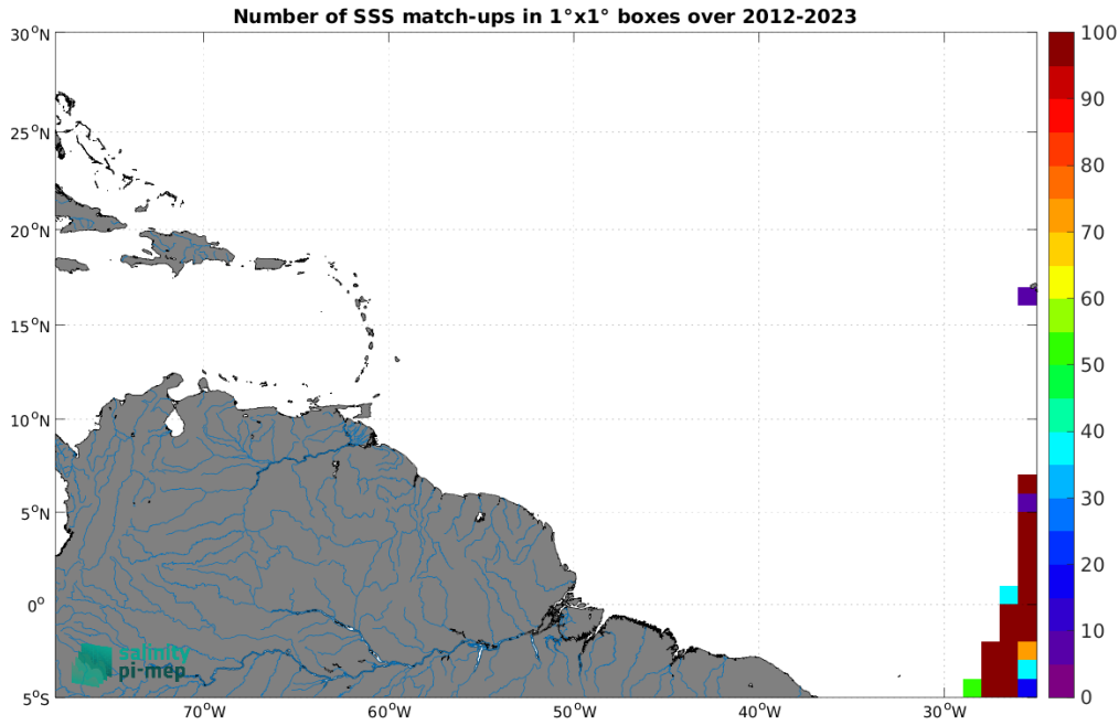
Figure 5: Number of SSS match-ups between TSG (Polarstern) SSS and the SMOS SSS L4 OI v346 - Weekly (CMEMS-CATDS-LOPS) SSS product for the Amazon and Orinoco river plumes Pi-MEP region over 1^\circ \times 1^\circ boxes and for the full satellite product period.
