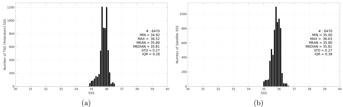
Figure 3: Histograms of SSS from TSG (Polarstern) (a) and SMOS SSS L4 OI v346 - Weekly (CMEMS-CATDS-LOPS) (b) considering all match-up pairs per bins of 0.1 over the Amazon and Orinoco river plumes Pi-MEP region and for the full satellite product period.
