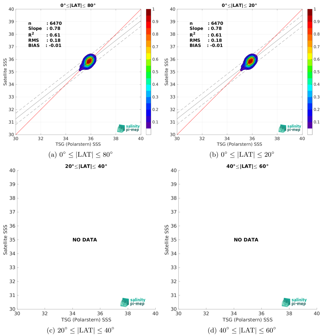
Figure 10: Contour maps of the concentration of SMOS SSS L4 OI v346 - Weekly (CMEMS-CATDS-LOPS) SSS (y-axis) versus TSG (Polarstern) SSS (x-axis) at match-up pairs for different latitude bands. For each plot, the red line shows x=y . The black thin and dashed lines indicate a linear fit through the data cloud and the \pm 95\% confidence levels, respectively. The number match-up pairs n , the slope and R^2 coefficient of the linear fit, the root mean square (RMS) and the mean bias between satellite and in situ data are indicated for each latitude band in each plots.
