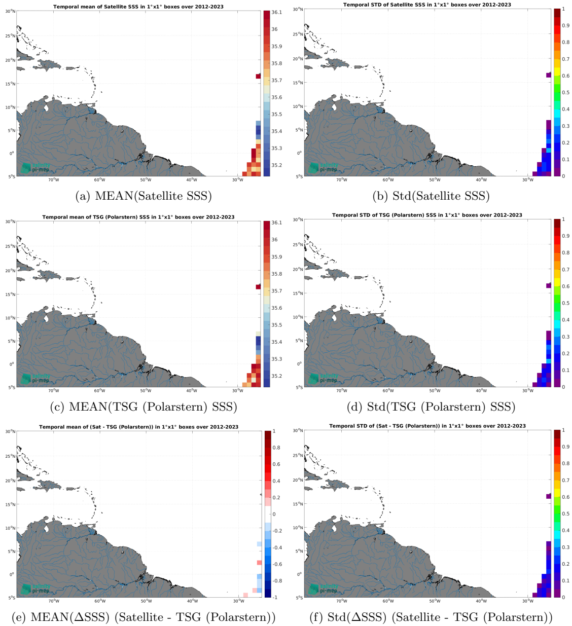
Figure 7: Temporal mean (left) and Std (right) of SSS from SMOS SSS L4 OI v346 - Weekly (CMEMS-CATDS-LOPS) (top), TSG (Polarstern) (middle), and of \Delta SSS (Satellite - TSG (Polarstern)). Only match-up pairs are used to generate these maps.
