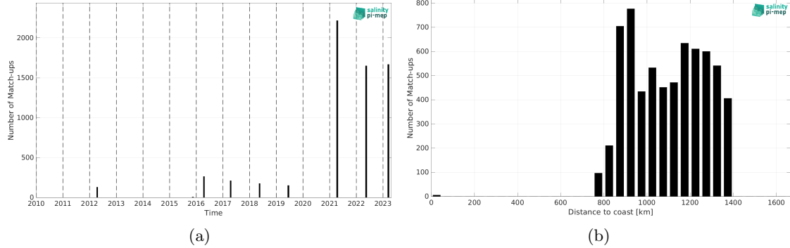
Figure 2: Number of match-ups between TSG (Polarstern) and SMOS SSS L4 OI v346 - Weekly (CMEMS-CATDS-LOPS) SSS as a function of time (a) and as function of the distance to coast (b) over the Amazon and Orinoco river plumes Pi-MEP region and for the full satellite product period.
