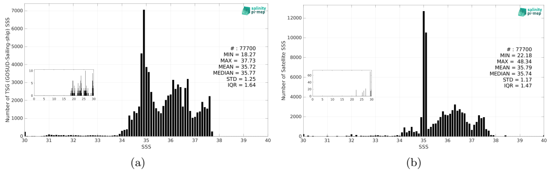
Figure 3: Histograms of SSS from TSG (GOSUD-Sailing-ship) (a) and SMOS SSS L4 OI v346 - Weekly (CMEMS-CATDS-LOPS) (b) considering all match-up pairs per bins of 0.1 over the Amazon and Orinoco river plumes Pi-MEP region and for the full satellite product period.
