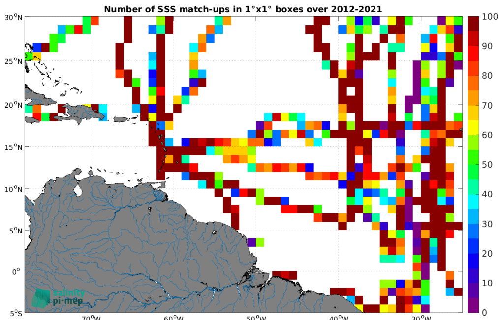
Figure 5: Number of SSS match-ups between TSG (GOSUD-Sailing-ship) SSS and the SMOS SSS L4 OI v346 - Weekly (CMEMS-CATDS-LOPS) SSS product for the Amazon and Orinoco river plumes Pi-MEP region over 1^\circ \times 1^\circ boxes and for the full satellite product period.
