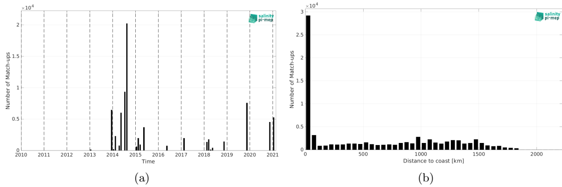
Figure 2: Number of match-ups between TSG (GOSUD-Sailing-ship) and SMOS SSS L4 OI v346 - Weekly (CMEMS-CATDS-LOPS) SSS as a function of time (a) and as function of the distance to coast (b) over the Amazon and Orinoco river plumes Pi-MEP region and for the full satellite product period.
