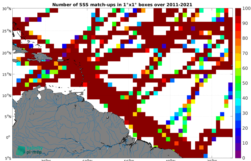
Figure 5: Number of SSS match-ups between TSG (GOSUD-Research-vessel) SSS and the SMOS SSS L4 OI v346 - Weekly (CMEMS-CATDS-LOPS) SSS product for the Amazon and Orinoco river plumes Pi-MEP region over 1°x1° boxes and for the full satellite product period.
