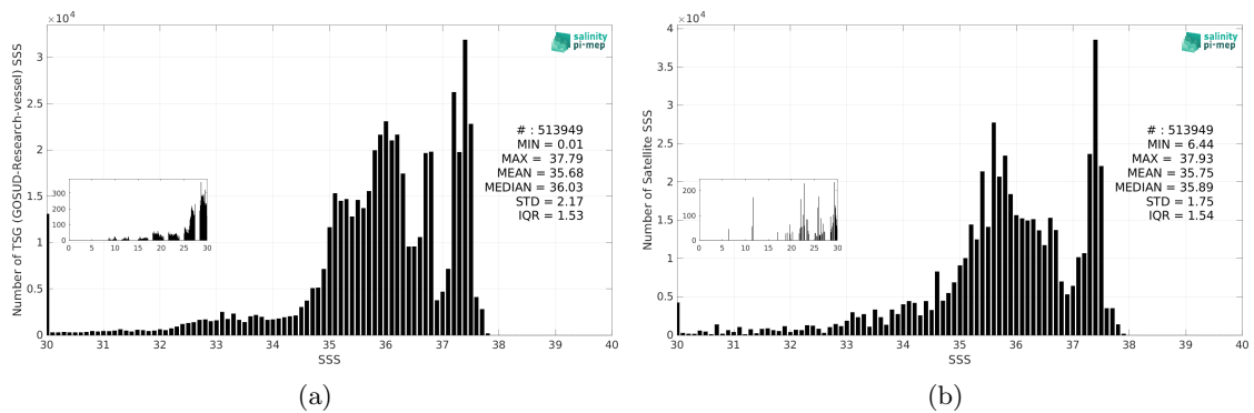
Figure 3: Histograms of SSS from TSG (GOSUD-Research-vessel) (a) and SMOS SSS L4 OI v346 - Weekly (CMEMS-CATDS-LOPS) (b) considering all match-up pairs per bins of 0.1 over the Amazon and Orinoco river plumes Pi-MEP region and for the full satellite product period.
