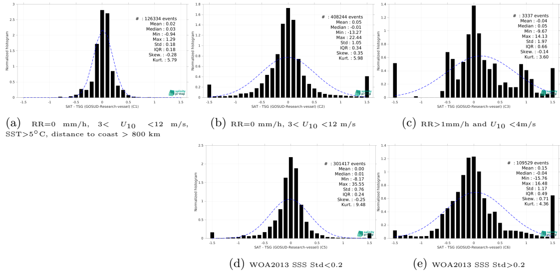
Figure 15: Normalized histogram of \Delta\text{SSS} (SMOS SSS L4 OI v346 - Weekly (CMEMS-CATDS-LOPS) - TSG (GOSUD-Research-vessel)) for 5 different subdatasets corresponding to: RR=0 mm/h, 3 < U_{10} < 12 m/s, SST > 5^\circ\text{C} , distance to coast > 800 km (a), RR=0 mm/h, 3 < U_{10} < 12 m/s (b), RR > 1 mm/h and U_{10} < 4 m/s (c), WOA2013 SSS Std < 0.2 (d), WOA2013 SSS Std > 0.2 (e).
