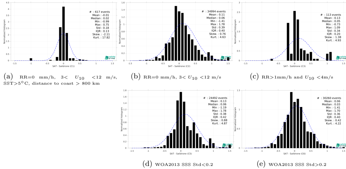
Figure 15: Normalized histogram of \Delta SSS (SMOS SSS L4 OI v346 - Weekly (CMEMS-CATDS-LOPS) - Sairdrone) for 5 different subdatasets corresponding to: RR=0 mm/h, 3 < U_{10} < 12 m/s, SST>5°C, distance to coast > 800 km (a), RR=0 mm/h, 3 < U_{10} < 12 m/s (b), RR>1mm/h and U_{10} < 4 m/s (c), WOA2013 SSS Std<0.2 (d), WOA2013 SSS Std>0.2 (e).
