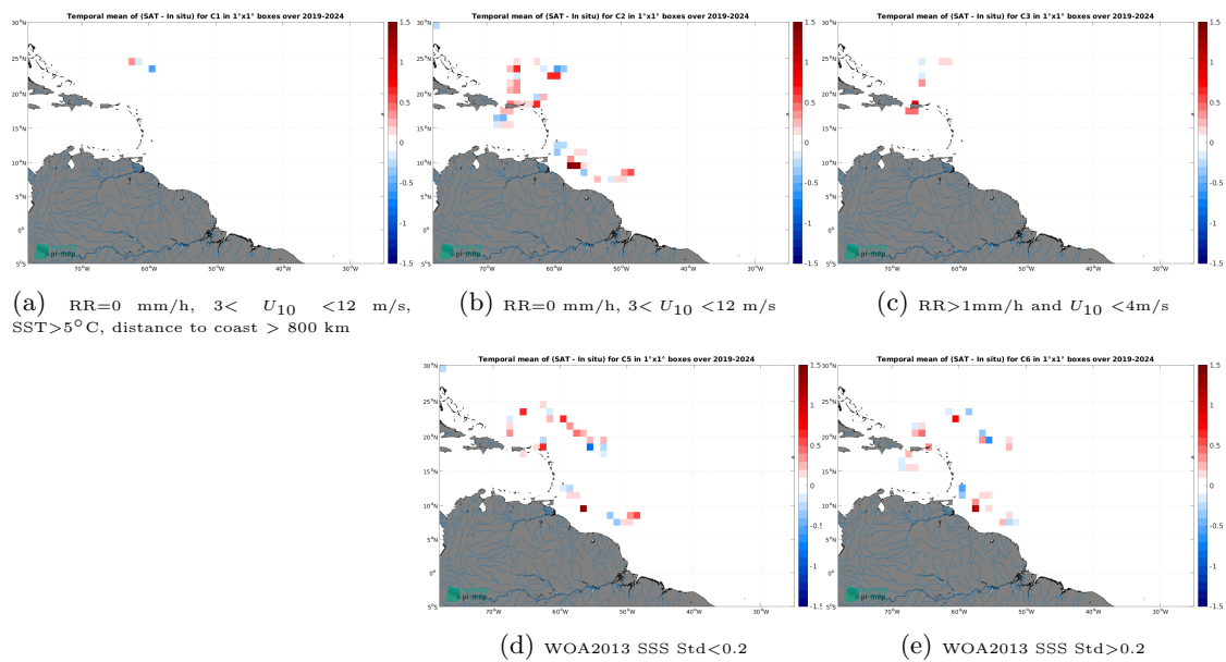
Figure 14: Temporal mean gridded over spatial boxes of size 1^\circ \times 1^\circ of \Delta SSS (SMOS SSS L4 OI v346 - Weekly (CMEMS-CATDS-LOPS) - Saildrone) for 5 different subdatasets corresponding to:RR=0 mm/h, 3 < U_{10} < 12 m/s, SST >5^\circ\text{C} , distance to coast > 800 km (a), RR=0 mm/h, 3 < U_{10} < 12 m/s (b), RR >1 mm/h and U_{10} < 4 m/s (c), WOA2013 SSS Std <0.2 (d), WOA2013 SSS Std >0.2 (e).
