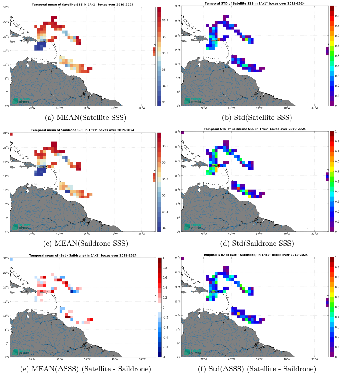
Figure 7: Temporal mean (left) and Std (right) of SSS from SMOS SSS L4 OI v346 - Weekly (CMEMS-CATDS-LOPS) (top), Saildrone (middle), and of \Delta SSS (Satellite - Saildrone). Only match-up pairs are used to generate these maps.
