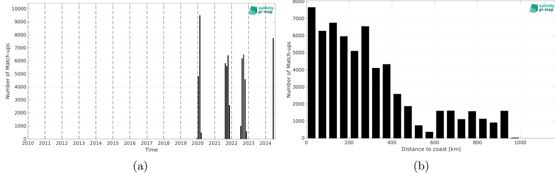
Figure 2: Number of match-ups between Saildrone and SMOS SSS L4 OI v346 - Weekly (CMEMS-CATDS-LOPS) SSS as a function of time (a) and as function of the distance to coast (b) over the Amazon and Orinoco river plumes Pi-MEP region and for the full satellite product period.
