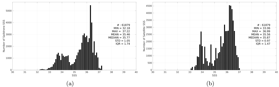
Figure 3: Histograms of SSS from Saildrone (a) and SMOS SSS L4 OI v346 - Weekly (CMEMS-CATDS-LOPS) (b) considering all match-up pairs per bins of 0.1 over the Amazon and Orinoco river plumes Pi-MEP region and for the full satellite product period.
