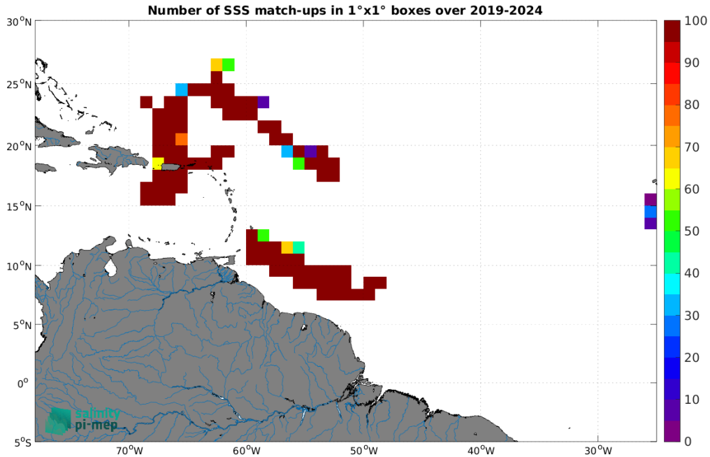
Figure 5: Number of SSS match-ups between Saildrone SSS and the SMOS SSS L4 OI v346 - Weekly (CMEMS-CATDS-LOPS) SSS product for the Amazon and Orinoco river plumes Pi-MEP region over 1^\circ \times 1^\circ boxes and for the full satellite product period.
