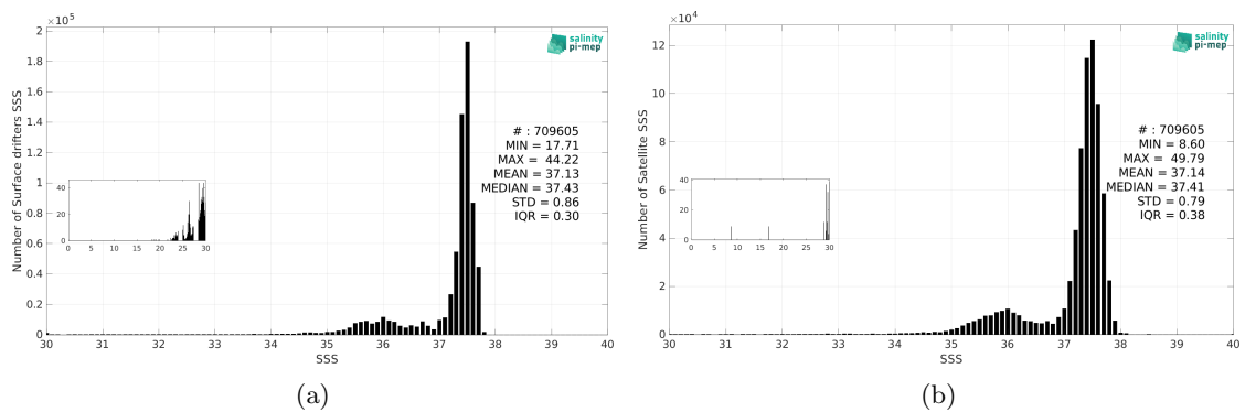
Figure 3: Histograms of SSS from Surface drifters (a) and SMOS SSS L4 OI v346 - Weekly (CMEMS-CATDS-LOPS) (b) considering all match-up pairs per bins of 0.1 over the Amazon and Orinoco river plumes Pi-MEP region and for the full satellite product period.
