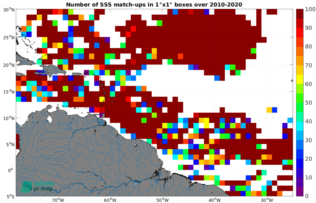
Figure 4: Number of SSS match-ups between Surface drifters SSS and the SMOS SSS L4 OI v346 - Weekly (CMEMS-CATDS-LOPS) SSS product for the Amazon and Orinoco river plumes Pi-MEP region over 1^\circ \times 1^\circ boxes and for the full satellite product period.
