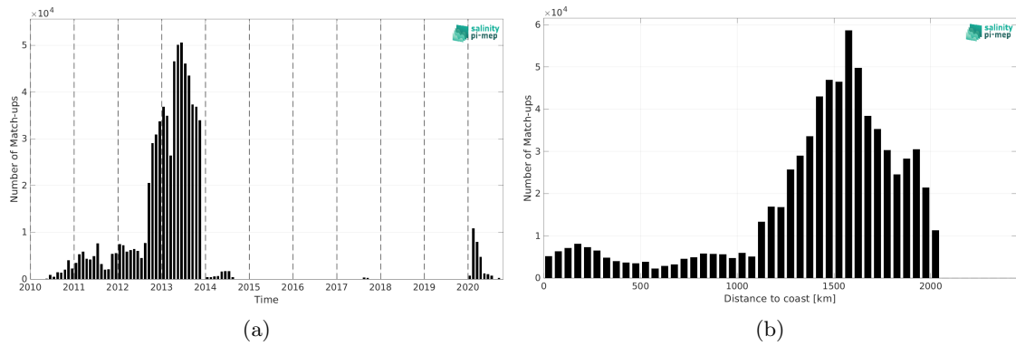
Figure 2: Number of match-ups between Surface drifters and SMOS SSS L4 OI v346 - Weekly (CMEMS-CATDS-LOPS) SSS as a function of time (a) and as function of the distance to coast (b) over the Amazon and Orinoco river plumes Pi-MEP region and for the full satellite product period.
