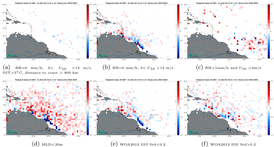
Figure 14: Temporal mean gridded over spatial boxes of size 1^\circ \times 1^\circ of \Delta SSS (SMOS SSS L4 OI v346 - Weekly (CMEMS-CATDS-LOPS) - Argo) for 6 different subdatasets corresponding to: RR=0 mm/h, 3 < U_{10} < 12 m/s, SST > 5^\circ C, distance to coast > 800 km (a), RR=0 mm/h, 3 < U_{10} < 12 m/s (b), RR > 1 mm/h and U_{10} < 4 m/s (c),MLD < 20 m (d),WOA2013 SSS Std < 0.2 (e),WOA2013 SSS Std > 0.2 (f).
