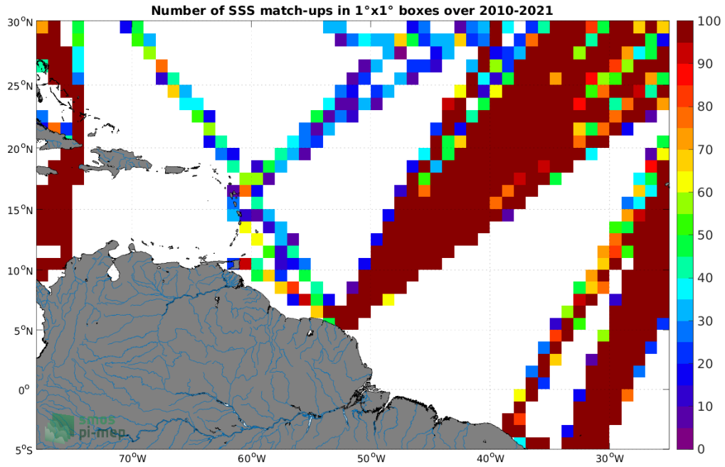
Figure 3: Number of SSS match-ups between TSG (LEGOS-DM) SSS and the SMOS SSS L4 OI v342 - Weekly (CMEMS-CATDS-LOPS) SSS product for the Amazon and Orinoco river plumes Pi-MEP region over 1^\circ \times 1^\circ boxes and for the full satellite product period.
