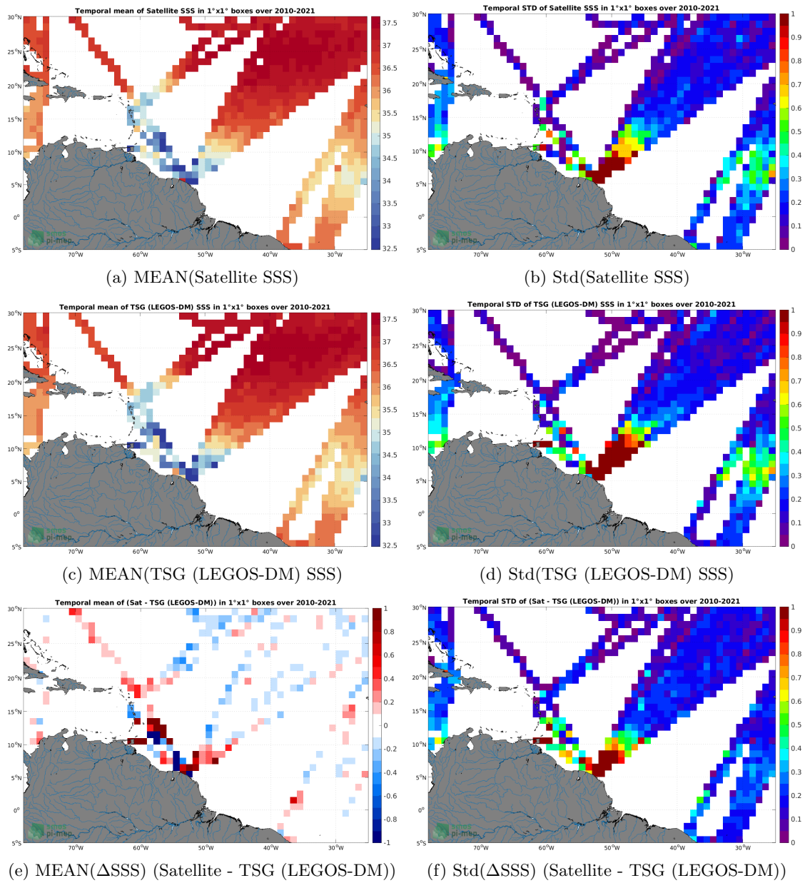
Figure 5: Temporal mean (left) and Std (right) of SSS from SMOS SSS L4 OI v342 - Weekly (CMEMS-CATDS-LOPS) (top), TSG (LEGOS-DM) (middle), and of \Delta SSS (Satellite - TSG (LEGOS-DM)). Only match-up pairs are used to generate these maps.
