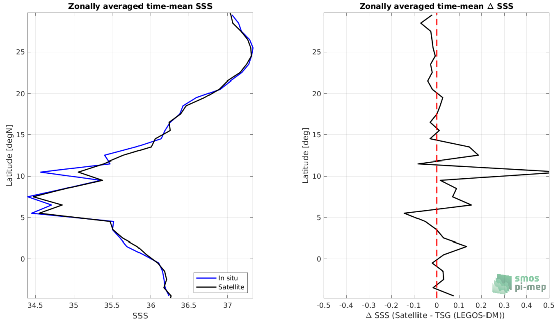
Figure 7: Left panel: Zonal mean SSS from SMOS SSS L4 OI v342 - Weekly (CMEMS-CATDS-LOPS) satellite product (black) and from TSG (LEGOS-DM) (blue). Right panel: Zonal mean of \Delta SSS (Satellite - TSG (LEGOS-DM)) for all the collected Pi-MEP match-up pairs estimated over the full satellite product period.
