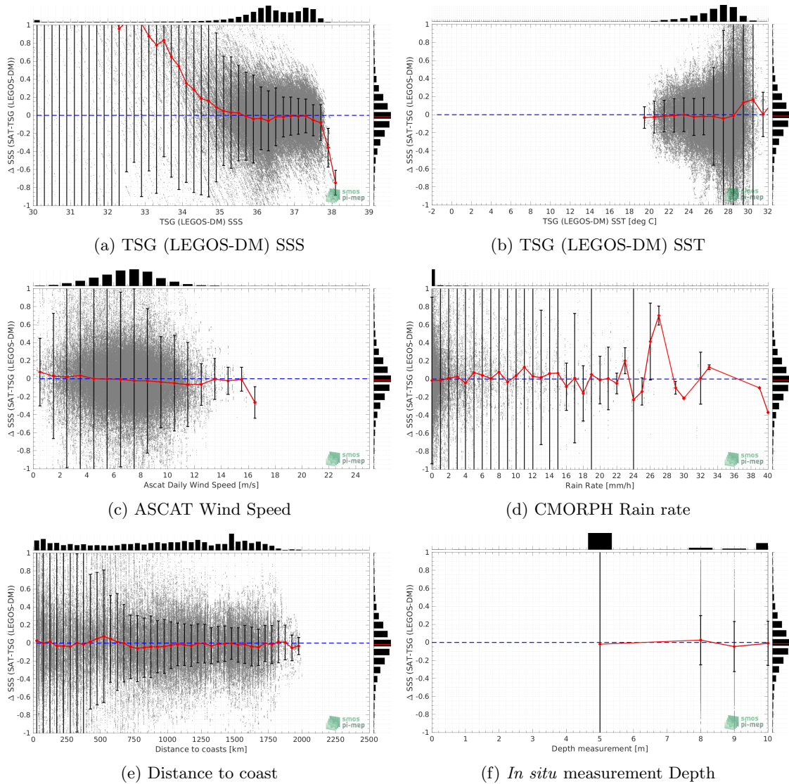
Figure 10: \Delta SSS (Satellite - TSG (LEGOS-DM)) sorted as function of TSG (LEGOS-DM) SSS values a), TSG (LEGOS-DM) SST b), ASCAT Wind speed c), CMORPH rain rate d), distance to coast (e) and in situ measurement depth (f). In all plots the median and Std of \Delta SSS for each bin is indicated by the red curves and black vertical thick bars ( \pm 1 Std)
