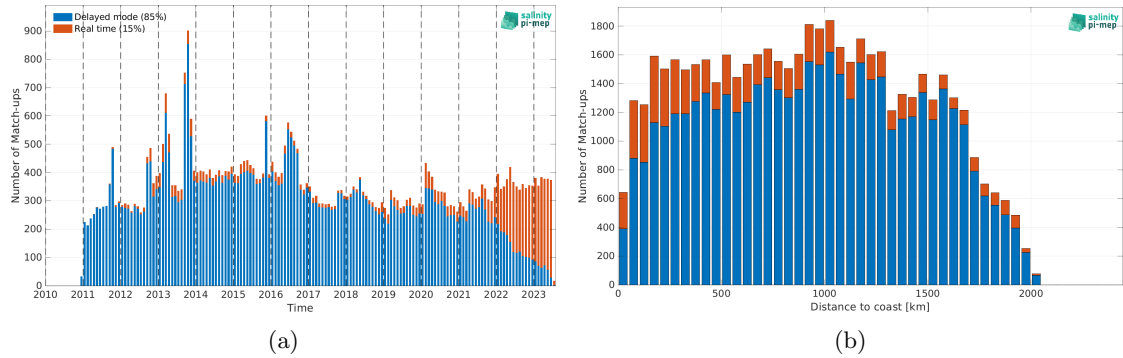
Figure 1: Number of match-ups between Argo and SMOS SSS L4 OI v342 - Weekly (CMEMS-CATDS-LOPS) SSS as a function of time (a) and as function of the distance to coast (b) over the Amazon and Orinoco river plumes Pi-MEP region and for the full satellite product period.
