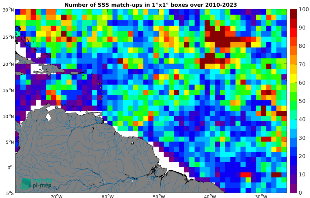
Figure 4: Number of SSS match-ups between Argo SSS and the SMOS SSS L4 OI v342 - Weekly (CMEMS-CATDS-LOPS) SSS product for the Amazon and Orinoco river plumes Pi-MEP region over 1^\circ \times 1^\circ boxes and for the full satellite product period.
