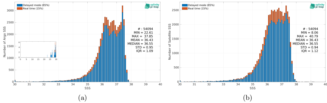
Figure 2: Histograms of SSS from Argo (a) and SMOS SSS L4 OI v342 - Weekly (CMEMS-CATDS-LOPS) (b) considering all match-up pairs per bins of 0.1 over the Amazon and Orinoco river plumes Pi-MEP region and for the full satellite product period.
