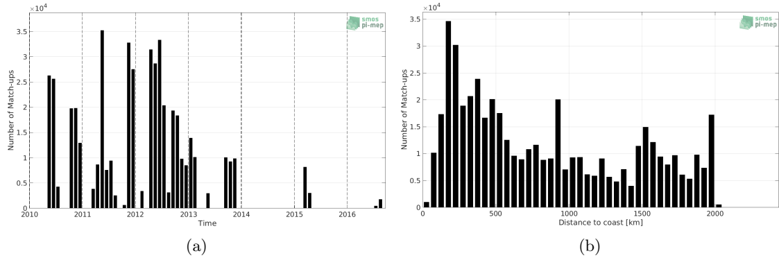
Figure 1: Number of match-ups between TSG (SAMOS) and SMOS L4 v2 Weekly (CATDS-CECOS-IFREMER) SSS as a function of time (a) and as function of the distance to coast (b) over the Amazon and Orinoco river plumes Pi-MEP region and for the full satellite product period.
