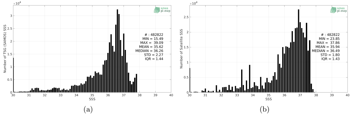
Figure 2: Histograms of SSS from TSG (SAMOS) (a) and SMOS L4 v2 Weekly (CATDS-CECOS-IFREMER) (b) considering all match-up pairs per bins of 0.1 over the Amazon and Orinoco river plumes Pi-MEP region and for the full satellite product period.
