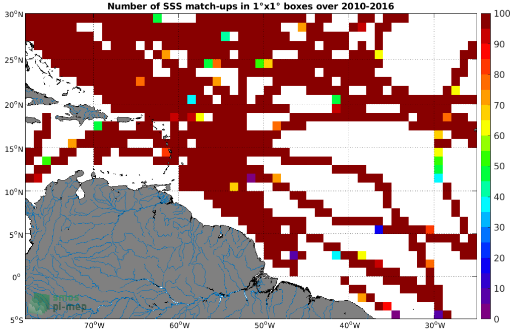
Figure 4: Number of SSS match-ups between TSG (SAMOS) SSS and the SMOS L4 v2 Weekly (CATDS-CECOS-IFREMER) SSS product for the Amazon and Orinoco river plumes Pi-MEP region over 1^\circ \times 1^\circ boxes and for the full satellite product period.
