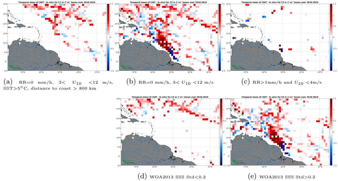
Figure 12: Temporal mean gridded over spatial boxes of size 1^{\circ}\times 1^{\circ} of \Delta\text{SSS} (SMOS L4 v2 Weekly (CATDS-CECOS-IFREMER) - TSG (SAMOS)) for 5 different subdatasets corresponding to: RR=0 mm/h, 3 < U_{10} < 12 m/s, SST > 5^{\circ}\text{C} , distance to coast > 800 km (a), RR=0 mm/h, 3 < U_{10} < 12 m/s (b), RR > 1 mm/h and U_{10} < 4 m/s (c), WOA2013 SSS Std < 0.2 (d), WOA2013 SSS Std > 0.2 (e).
