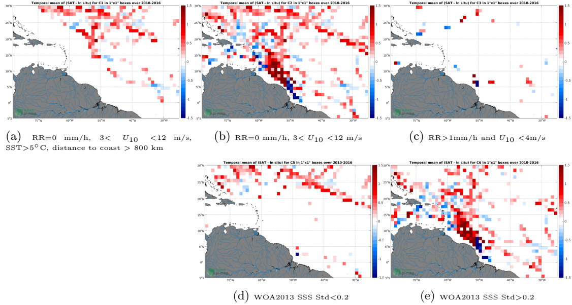
Figure 12: Temporal mean gridded over spatial boxes of size 1^{\circ}\times 1^{\circ} of \Delta\text{SSS} (SMOS-L4-CATDS-CECOS-IFREMER-V2-WEEKLY-0.5DEG - TSG-SAMOS) for 5 different subdatasets corresponding to: RR=0 mm/h, 3 < U_{10} < 12 m/s, SST >5^{\circ}\text{C} , distance to coast > 800 km (a), RR=0 mm/h, 3 < U_{10} < 12 m/s (b), RR >1 mm/h and U_{10} < 4 m/s (c), WOA2013 SSS Std <0.2 (d), WOA2013 SSS Std >0.2 (e).
