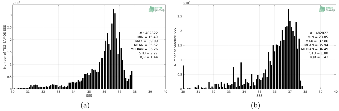
Figure 2: Histograms of SSS from TSG-SAMOS (a) and SMOS-L4-CATDS-CECOS-IFREMER-V2-WEEKLY-0.5DEG (b) considering all match-up pairs per bins of 0.1 over the Amazon and Orinoco river plumes Pi-MEP region and for the full satellite product period.
