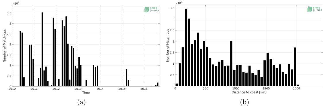
Figure 1: Number of match-ups between TSG-SAMOS and SMOS-L4-CATDS-CECOS-IFREMER-V2-WEEKLY-0.5DEG SSS as a function of time (a) and as function of the distance to coast (b) over the Amazon and Orinoco river plumes Pi-MEP region and for the full satellite product period.
