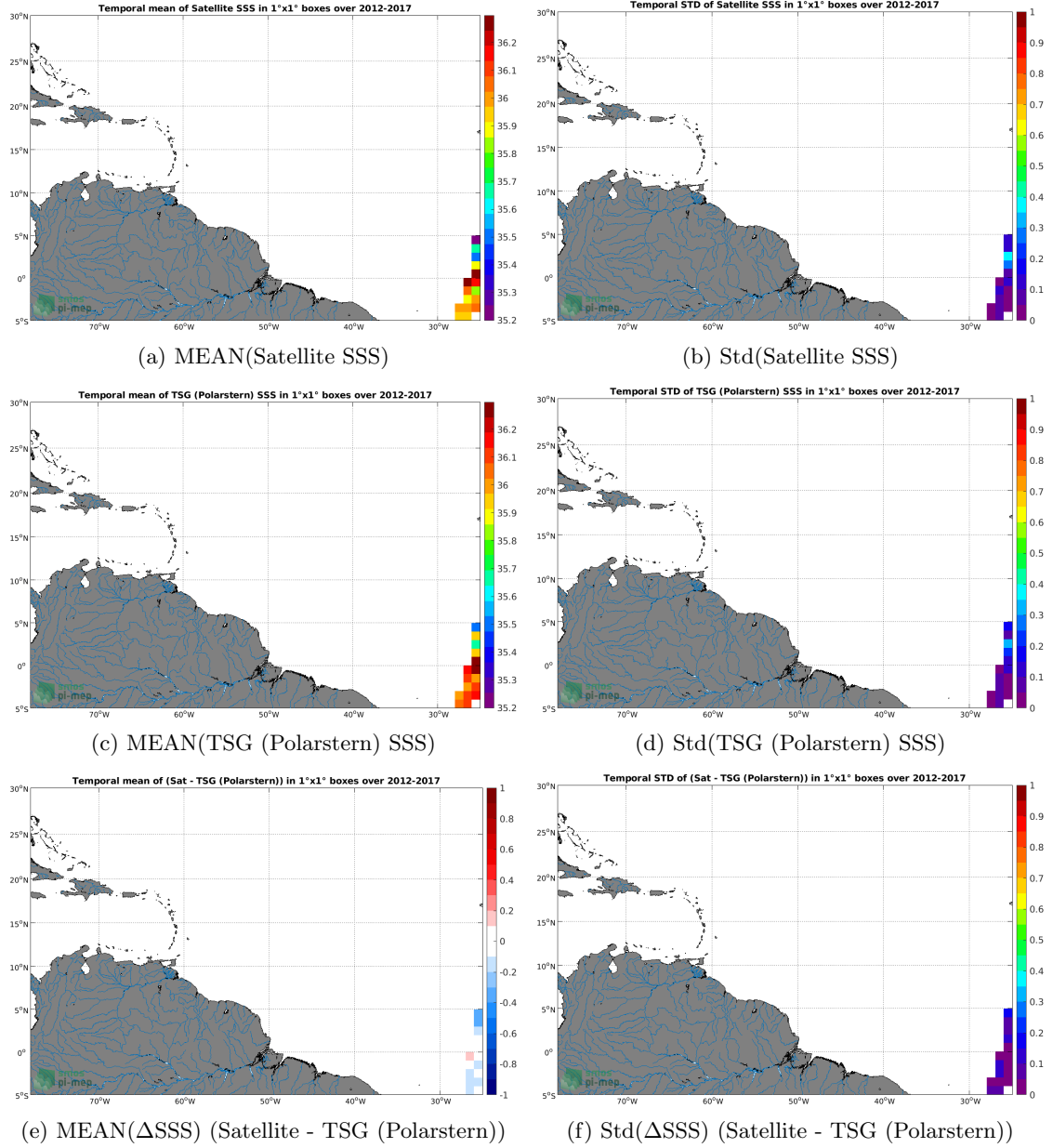
Figure 6: Temporal mean (left) and Std (right) of SSS from SMOS L4 v2 Weekly (CATDS-CECOS-IFREMER) (top), TSG (Polarstern) (middle), and of \Delta SSS (Satellite - TSG (Polarstern)). Only match-up pairs are used to generate these maps.
