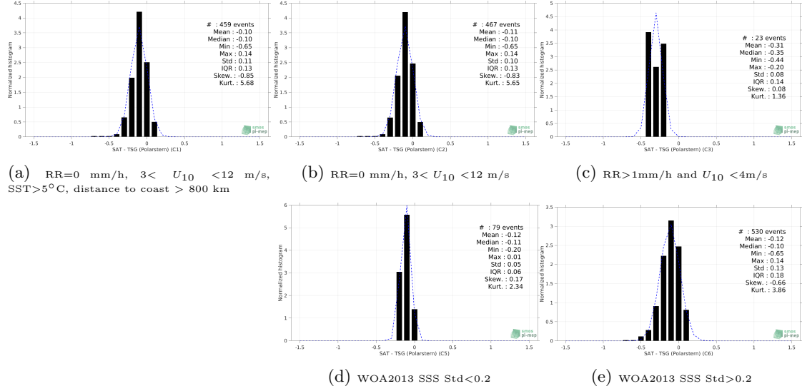
Figure 13: Normalized histogram of \Delta\text{SSS} (SMOS L4 v2 Weekly (CATDS-CECOS-IFREMER) - TSG (Polarstern)) for 5 different subdatasets corresponding to: RR=0 mm/h, 3 < U_{10} < 12 m/s, SST > 5^\circ\text{C} , distance to coast > 800 km (a), RR=0 mm/h, 3 < U_{10} < 12 m/s (b), RR > 1\text{mm/h} and U_{10} < 4\text{m/s} (c), WOA2013 SSS Std < 0.2 (d), WOA2013 SSS Std > 0.2 (e).
