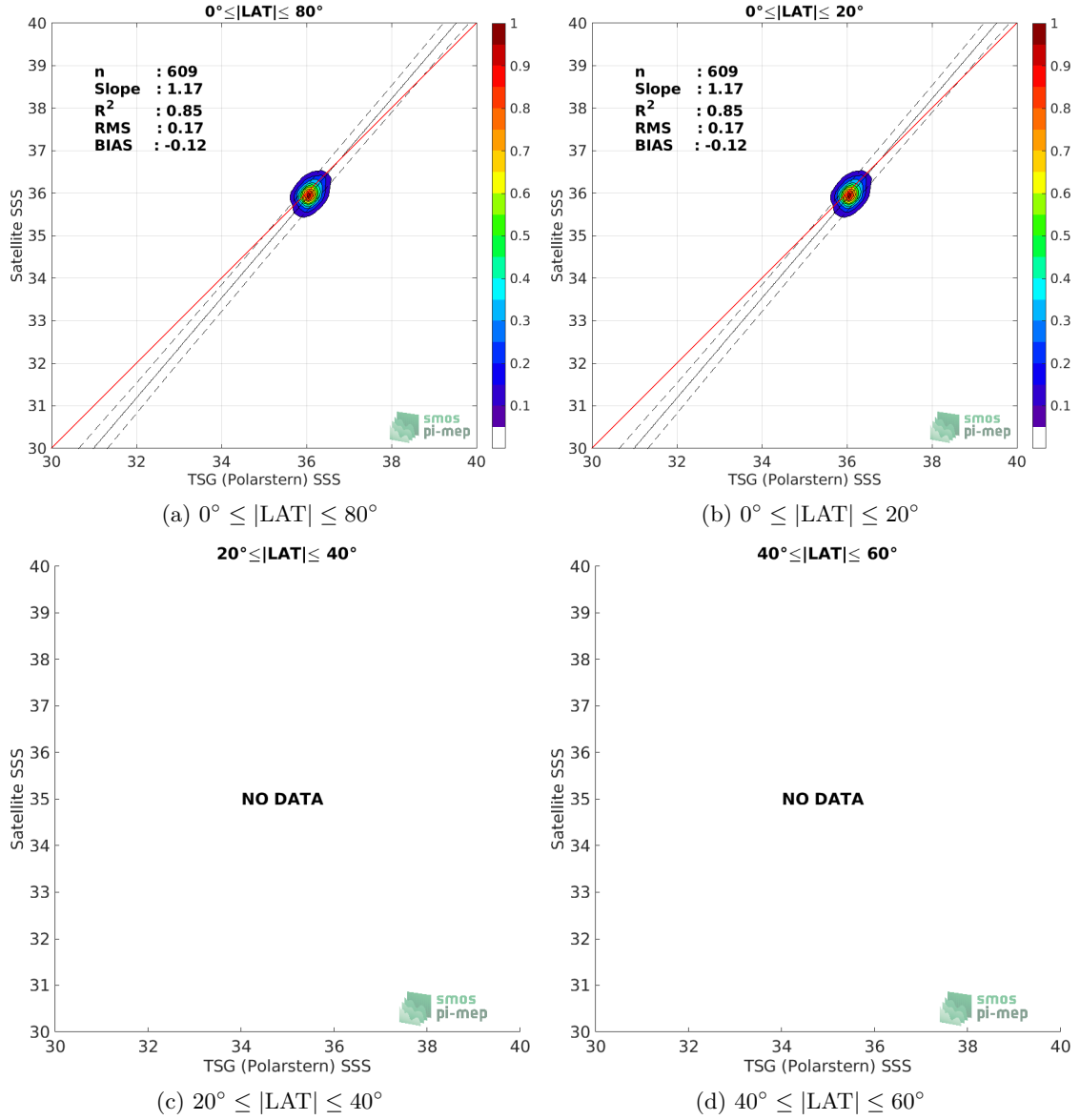
Figure 9: Contour maps of the concentration of SMOS L4 v2 Weekly (CATDS-CECOS-IFREMER) SSS (y-axis) versus TSG (Polarstern) SSS (x-axis) at match-up pairs for different latitude bands. For each plot, the red line shows x=y . The black thin and dashed lines indicate a linear fit through the data cloud and the \pm 95\% confidence levels, respectively. The number match-up pairs n , the slope and R^2 coefficient of the linear fit, the root mean square (RMS) and the mean bias between satellite and in situ data are indicated for each latitude band in each plots.
