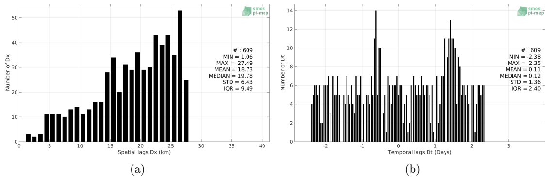
Figure 5: Histograms of the spatial (a) and temporal (b) lags between the location/time of the TSG (Polarstern) measurement and the date of the corresponding SMOS L4 v2 Weekly (CATDS-CECOS-IFREMER) SSS pixel.
