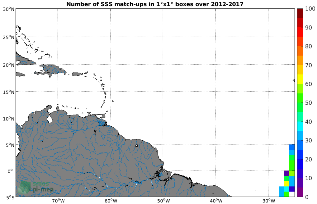
Figure 4: Number of SSS match-ups between TSG (Polarstern) SSS and the SMOS L4 v2 Weekly (CATDS-CECOS-IFREMER) SSS product for the Amazon and Orinoco river plumes Pi-MEP region over 1^\circ \times 1^\circ boxes and for the full satellite product period.
