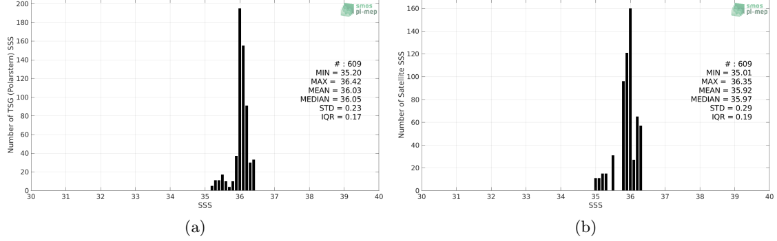
Figure 2: Histograms of SSS from TSG (Polarstern) (a) and SMOS L4 v2 Weekly (CATDS-CECOS-IFREMER) (b) considering all match-up pairs per bins of 0.1 over the Amazon and Orinoco river plumes Pi-MEP region and for the full satellite product period.
