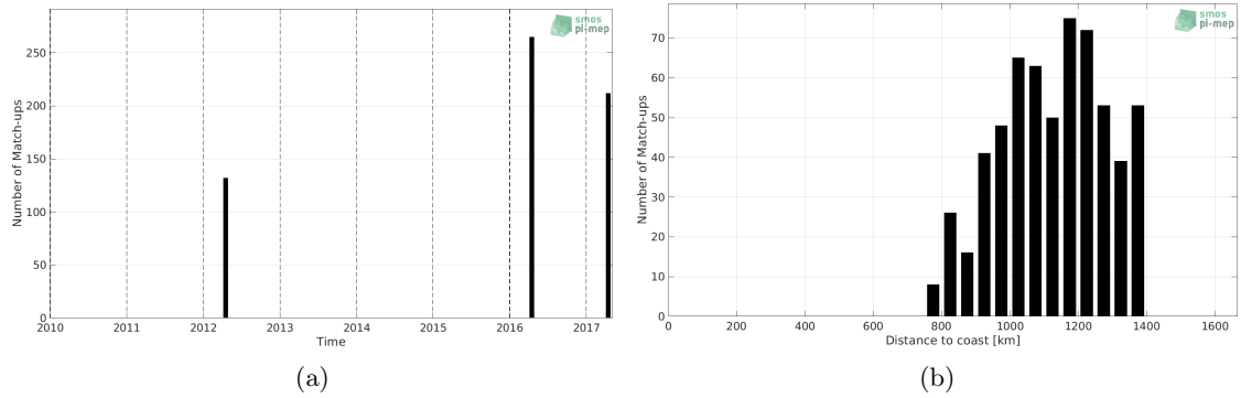
Figure 1: Number of match-ups between TSG (Polarstern) and SMOS L4 v2 Weekly (CATDS-CECOS-IFREMER) SSS as a function of time (a) and as function of the distance to coast (b) over the Amazon and Orinoco river plumes Pi-MEP region and for the full satellite product period.
