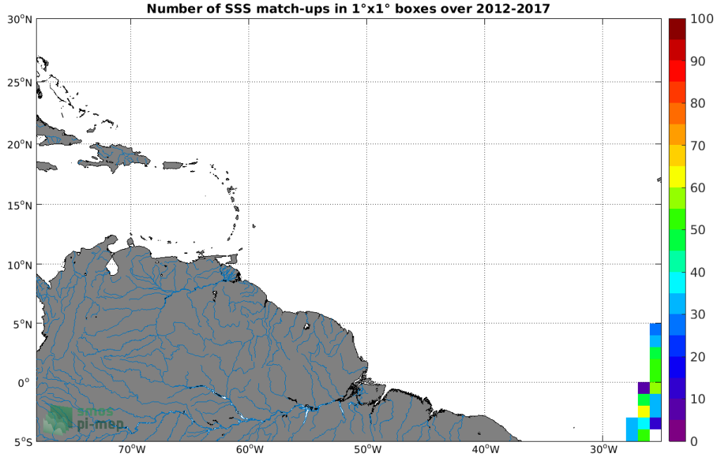
Figure 4: Number of SSS match-ups between TSG (Polarstern) SSS and the SMOS L4 v2 Weekly (CATDS-CECOS-IFREMER) SSS product for the Amazon and Orinoco river plumes Pi-MEP region over 1°x1° boxes and for the full satellite product period.
