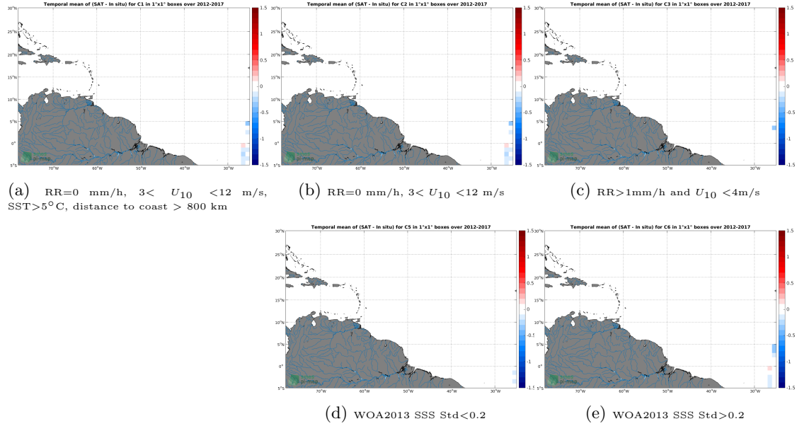
Figure 12: Temporal mean gridded over spatial boxes of size 1^{\circ}\times 1^{\circ} of \Delta\text{SSS} (SMOS-L4-CATDS-CECOS-IFREMER-V2-WEEKLY-0.5DEG - TSG-POLARSTERN) for 5 different subdatasets corresponding to: RR=0 mm/h, 3 < U_{10} < 12 m/s, SST >5^{\circ}\text{C} , distance to coast > 800 km (a), RR=0 mm/h, 3 < U_{10} < 12 m/s (b), RR >1 mm/h and U_{10} < 4 m/s (c), WOA2013 SSS Std <0.2 (d), WOA2013 SSS Std >0.2 (e).
