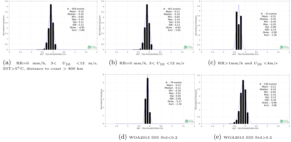
Figure 13: Normalized histogram of \Delta SSS (SMOS-L4-CATDS-CECOS-IFREMER-V2-WEEKLY-0.5DEG - TSG-POLARSTERN) for 5 different subdatasets corresponding to: RR=0 mm/h, 3 < U_{10} < 12 m/s, SST>5°C, distance to coast > 800 km (a), RR=0 mm/h, 3 < U_{10} < 12 m/s (b), RR>1mm/h and U_{10} < 4 m/s (c), WOA2013 SSS Std<0.2 (d), WOA2013 SSS Std>0.2 (e).
