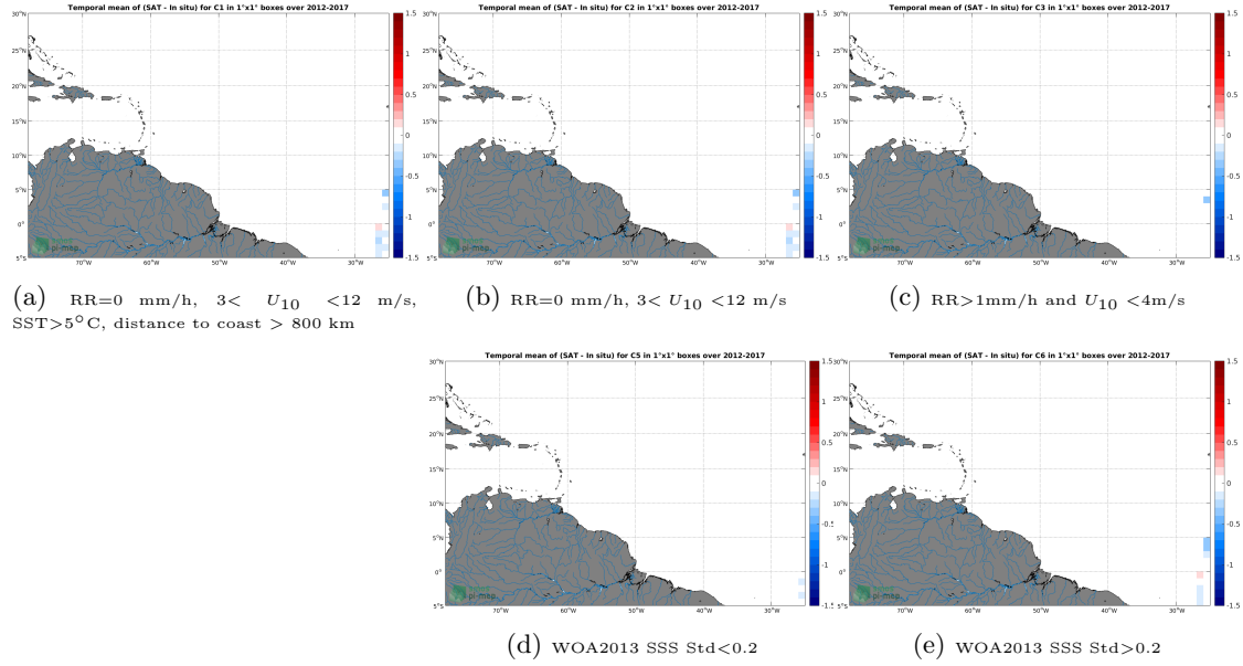
Figure 12: Temporal mean gridded over spatial boxes of size 1^\circ \times 1^\circ of \Delta SSS (SMOS-L4-CATDS-CECOS-IFREMER-V2-WEEKLY-0.5DEG - TSG-POLARSTERN) for 5 different subdatasets corresponding to: RR=0 mm/h, 3 < U_{10} < 12 m/s, SST > 5^\circ C , distance to coast > 800 km (a), RR=0 mm/h, 3 < U_{10} < 12 m/s (b), RR > 1 mm/h and U_{10} < 4 m/s (c), WOA2013 SSS Std < 0.2 (d), WOA2013 SSS Std > 0.2 (e).
