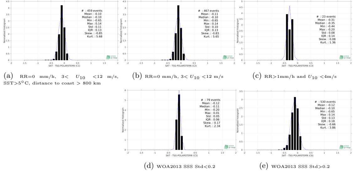
Figure 13: Normalized histogram of \Delta SSS (SMOS-L4-CATDS-CECOS-IFREMER-V2-WEEKLY-0.5DEG - TSG-POLARSTERN) for 5 different subdatasets corresponding to: RR=0 mm/h, 3 < U_{10} < 12 m/s, SST > 5^\circ C , distance to coast > 800 km (a), RR=0 mm/h, 3 < U_{10} < 12 m/s (b), RR > 1 mm/h and U_{10} < 4 m/s (c), WOA2013 SSS Std < 0.2 (d), WOA2013 SSS Std > 0.2 (e).
