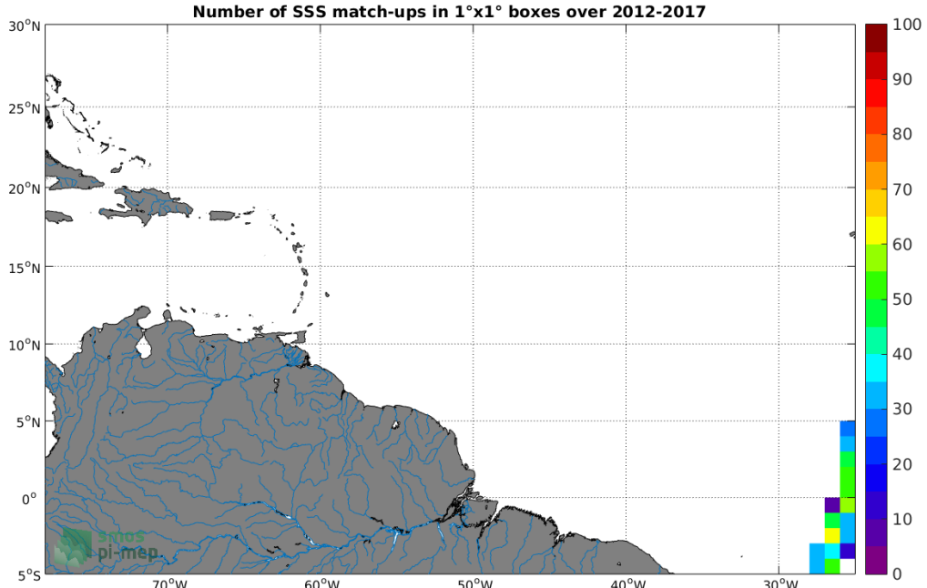
Figure 4: Number of SSS match-ups between TSG-POLARSTERN SSS and the SMOS-L4-CATDS-CECOS-IFREMER-V2-WEEKLY-0.5DEG SSS product for the Amazon and Orinoco river plumes Pi-MEP region over 1^\circ \times 1^\circ boxes and for the full satellite product period.
