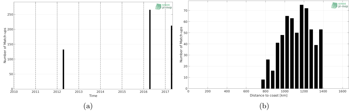
Figure 1: Number of match-ups between TSG-POLARSTERN and SMOS-L4-CATDS-CECOS-IFREMER-V2-WEEKLY-0.5DEG SSS as a function of time (a) and as function of the distance to coast (b) over the Amazon and Orinoco river plumes Pi-MEP region and for the full satellite product period.
