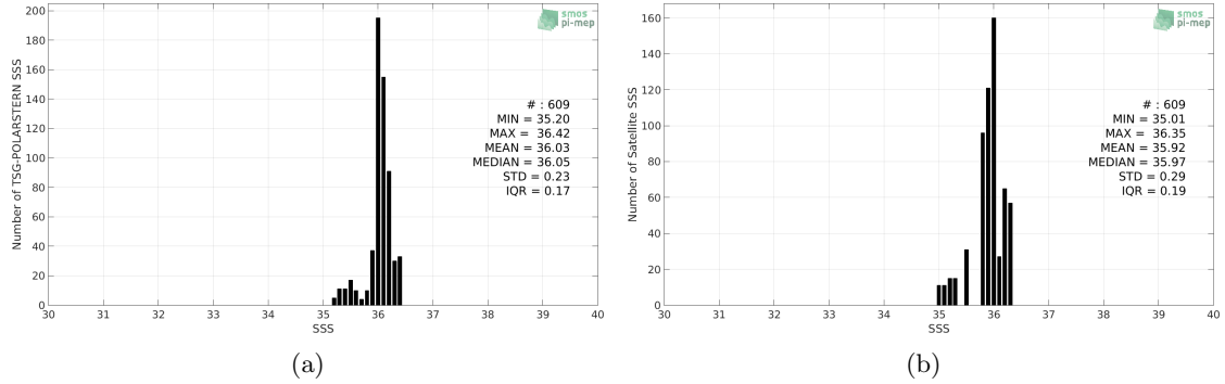
Figure 2: Histograms of SSS from TSG-POLARSTERN (a) and SMOS-L4-CATDS-CECOS-IFREMER-V2-WEEKLY-0.5DEG (b) considering all match-up pairs per bins of 0.1 over the Amazon and Orinoco river plumes Pi-MEP region and for the full satellite product period.
