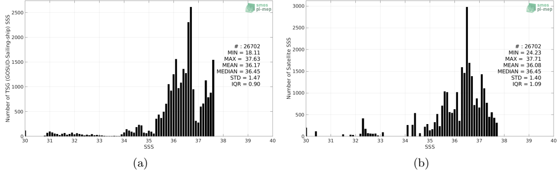
Figure 2: Histograms of SSS from TSG (GOSUD-Sailing-ship) (a) and SMOS L4 v2 Weekly (CATDS-CECOS-IFREMER) (b) considering all match-up pairs per bins of 0.1 over the Amazon and Orinoco river plumes Pi-MEP region and for the full satellite product period.
