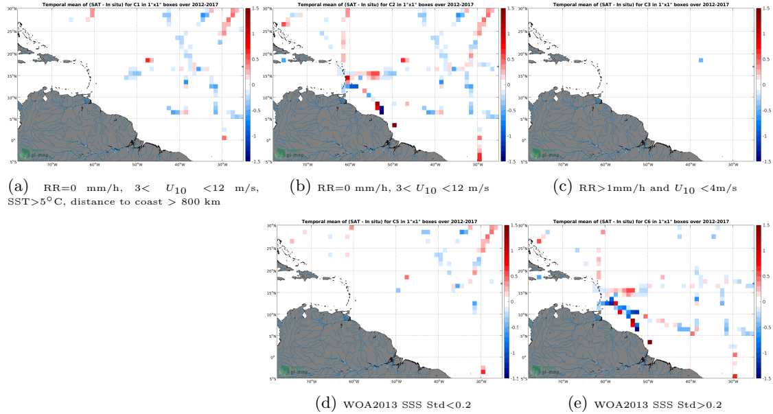
Figure 12: Temporal mean gridded over spatial boxes of size 1^{\circ}\times 1^{\circ} of \Delta SSS (SMOS L4 v2 Weekly (CATDS-CECOS-IFREMER) - TSG (GOSUD-Sailing-ship)) for 5 different subdatasets corresponding to: RR=0 mm/h, 3 < U_{10} < 12 m/s, SST >5^{\circ}\text{C} , distance to coast > 800 km (a), RR=0 mm/h, 3 < U_{10} < 12 m/s (b), RR>1 mm/h and U_{10} < 4 m/s (c), WOA2013 SSS Std <0.2 (d), WOA2013 SSS Std >0.2 (e).
