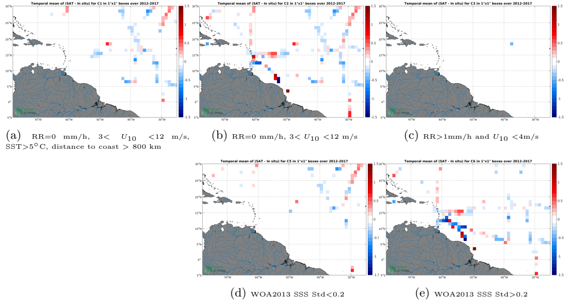
Figure 12: Temporal mean gridded over spatial boxes of size 1^\circ \times 1^\circ of \Delta SSS (SMOS-L4-CATDS-CECOS-IFREMER-V2-WEEKLY-0.5DEG - TSG-GOSUD-Sailing-ship) for 5 different subdatasets corresponding to: RR=0 mm/h, 3 < U_{10} < 12 m/s, SST >5^\circ\text{C} , distance to coast > 800 km (a), RR=0 mm/h, 3 < U_{10} < 12 m/s (b), RR >1 mm/h and U_{10} < 4 m/s (c), WOA2013 SSS Std <0.2 (d), WOA2013 SSS Std >0.2 (e).
