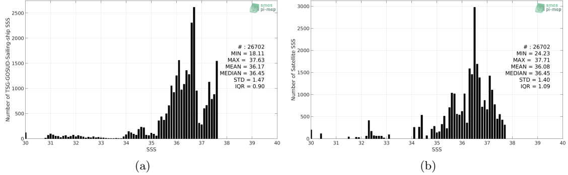
Figure 2: Histograms of SSS from TSG-GOSUD-Sailing-ship (a) and SMOS-L4-CATDS-CECOS-IFREMER-V2-WEEKLY-0.5DEG (b) considering all match-up pairs per bins of 0.1 over the Amazon and Orinoco river plumes Pi-MEP region and for the full satellite product period.
