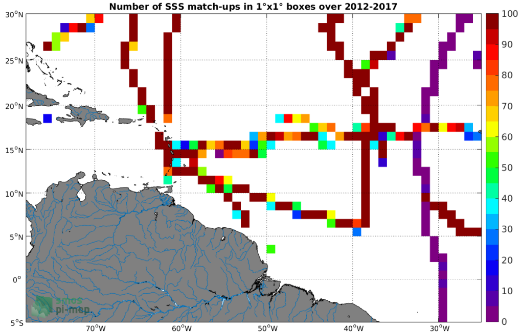
Figure 4: Number of SSS match-ups between TSG-GOSUD-Sailing-ship SSS and the SMOS-L4-CATDS-CECOS-IFREMER-V2-WEEKLY-0.5DEG SSS product for the Amazon and Orinoco river plumes Pi-MEP region over 1^\circ \times 1^\circ boxes and for the full satellite product period.
