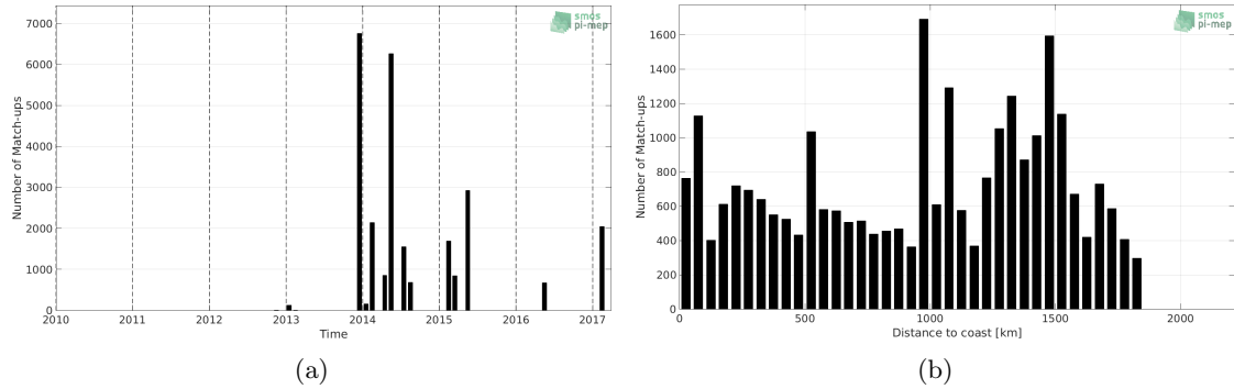
Figure 1: Number of match-ups between TSG-GOSUD-Sailing-ship and SMOS-L4-CATDS-CECOS-IFREMER-V2-WEEKLY-0.5DEG SSS as a function of time (a) and as function of the distance to coast (b) over the Amazon and Orinoco river plumes Pi-MEP region and for the full satellite product period.
