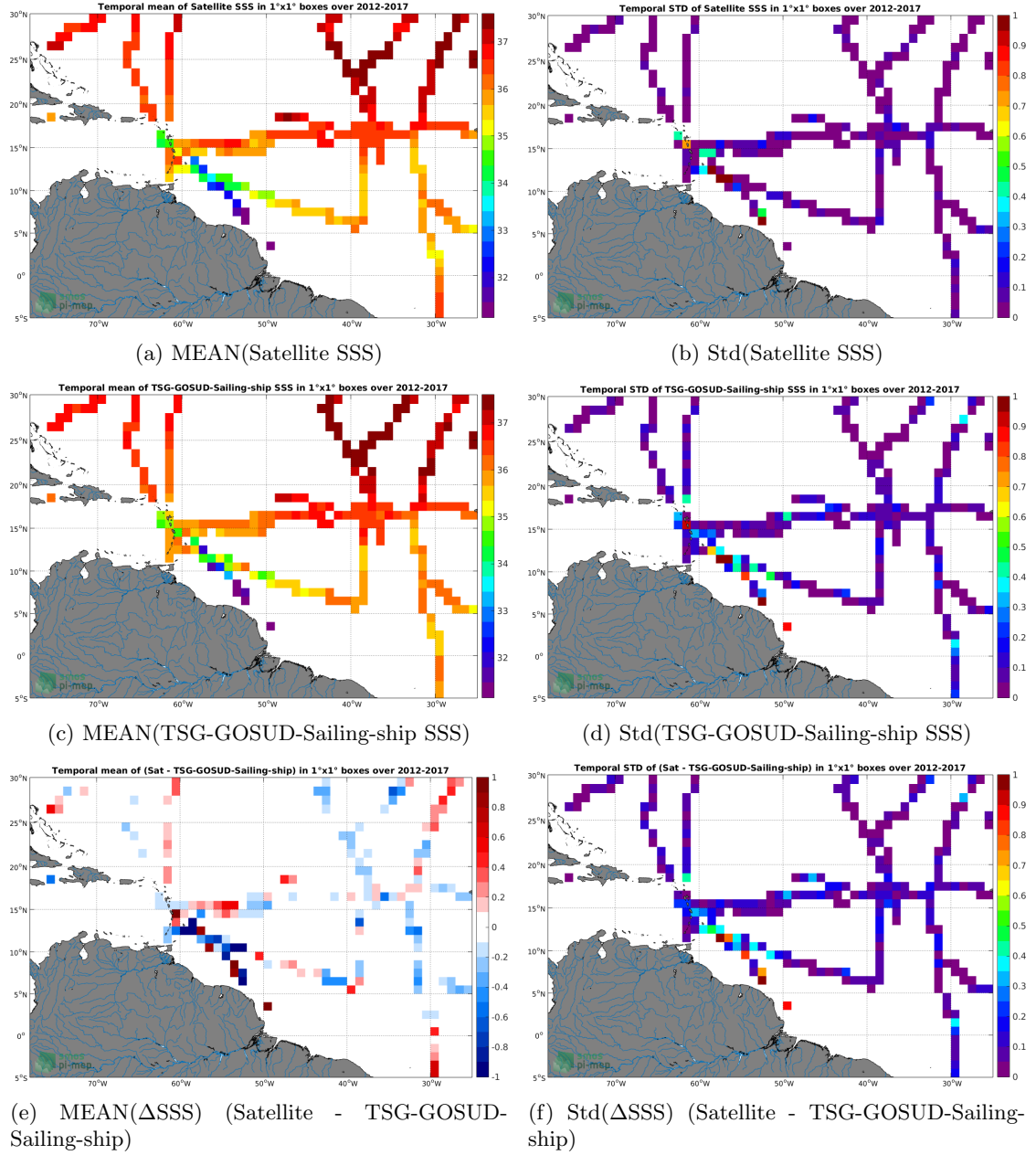
Figure 6: Temporal mean (left) and Std (right) of SSS from SMOS-L4-CATDS-CECOS-IFREMER-V2-WEEKLY-0.5DEG (top), TSG-GOSUD-Sailing-ship (middle), and of \Delta SSS (Satellite - TSG-GOSUD-Sailing-ship). Only match-up pairs are used to generate these maps.
