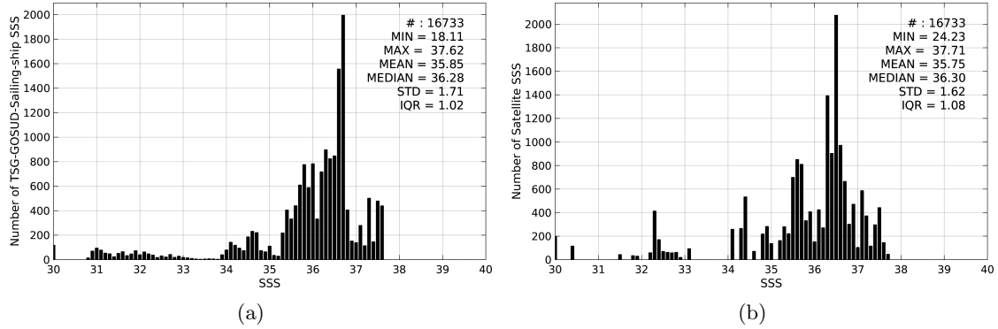
Figure 2: Histograms of SSS from TSG-GOSUD-Sailing-ship (a) and SMOS-L4-CATDS-CECOS-IFREMER-V2-WEEKLY-0.5DEG (b) considering all match-up pairs per bins of 0.1 over the Amazon and Orinoco river plumes Pi-MEP region and for the full satellite product period.
