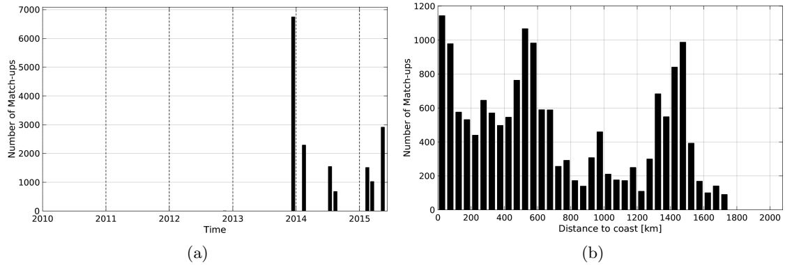
Figure 1: Number of match-ups between TSG-GOSUD-Sailing-ship and SMOS-L4-CATDS-CECOS-IFREMER-V2-WEEKLY-0.5DEG SSS as a function of time (a) and as function of the distance to coast (b) over the Amazon and Orinoco river plumes Pi-MEP region and for the full satellite product period.
