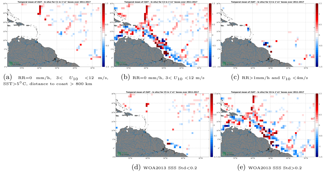
Figure 12: Temporal mean gridded over spatial boxes of size 1^{\circ}\times 1^{\circ} of \Delta SSS (SMOS-L4-CATDS-CECOS-IFREMER-V2-WEEKLY-0.5DEG - TSG-GOSUD-Research-vessel) for 5 different sub-datasets corresponding to: RR=0 mm/h, 3 < U_{10} < 12 m/s, SST >5^{\circ}\text{C} , distance to coast > 800 km (a), RR=0 mm/h, 3 < U_{10} < 12 m/s (b), RR >1 mm/h and U_{10} < 4 m/s (c), WOA2013 SSS Std <0.2 (d), WOA2013 SSS Std >0.2 (e).
