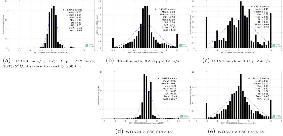
Figure 13: Normalized histogram of \Delta\text{SSS} (SMOS-L4-CATDS-CECOS-IFREMER-V2-WEEKLY-0.5DEG - TSG-GOSUD-Research-vessel) for 5 different subdatasets corresponding to: RR=0 mm/h, 3 < U_{10} < 12 m/s, SST > 5^\circ\text{C} , distance to coast > 800 km (a), RR=0 mm/h, 3 < U_{10} < 12 m/s (b), RR > 1\text{mm/h} and U_{10} < 4\text{m/s} (c), WOA2013 SSS Std < 0.2 (d), WOA2013 SSS Std > 0.2 (e).
