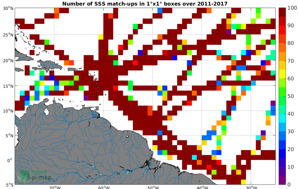
Figure 4: Number of SSS match-ups between TSG-GOSUD-Research-vessel SSS and the SMOS-L4-CATDS-CECOS-IFREMER-V2-WEEKLY-0.5DEG SSS product for the Amazon and Orinoco river plumes Pi-MEP region over 1^\circ \times 1^\circ boxes and for the full satellite product period.
