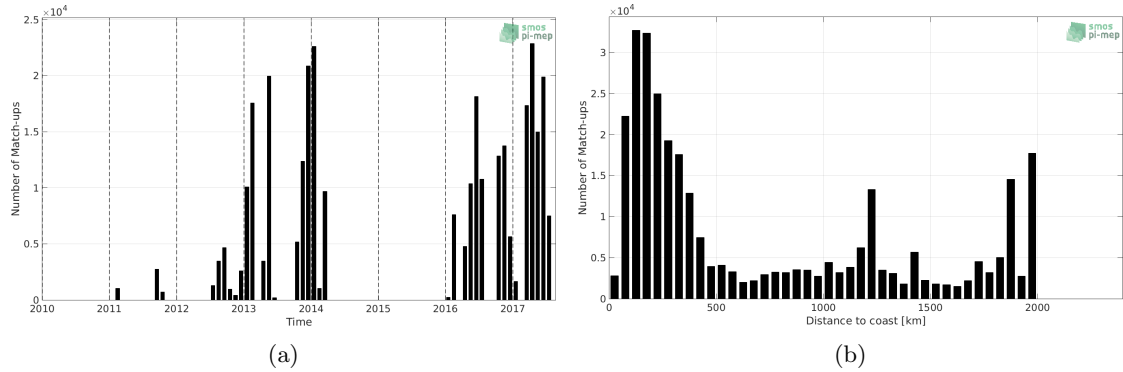
Figure 1: Number of match-ups between TSG-GOSUD-Research-vessel and SMOS-L4-CATDS-CECOS-IFREMER-V2-WEEKLY-0.5DEG SSS as a function of time (a) and as function of the distance to coast (b) over the Amazon and Orinoco river plumes Pi-MEP region and for the full satellite product period.
