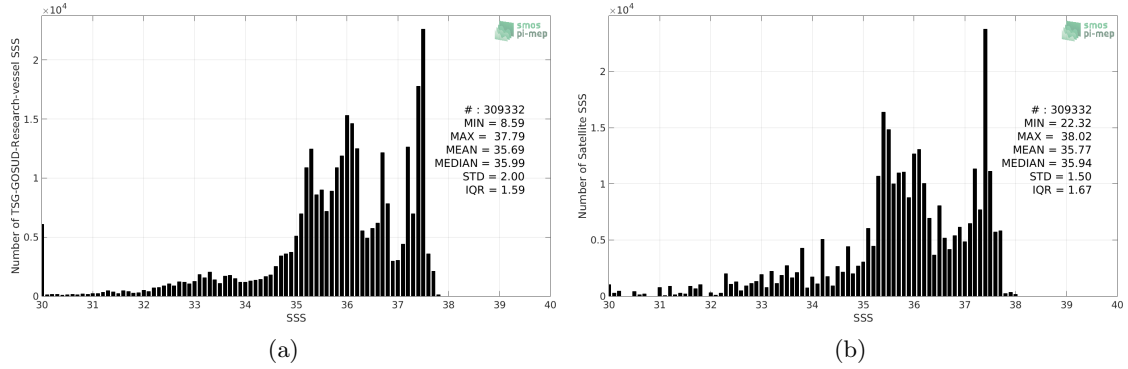
Figure 2: Histograms of SSS from TSG-GOSUD-Research-vessel (a) and SMOS-L4-CATDS-CECOS-IFREMER-V2-WEEKLY-0.5DEG (b) considering all match-up pairs per bins of 0.1 over the Amazon and Orinoco river plumes Pi-MEP region and for the full satellite product period.
