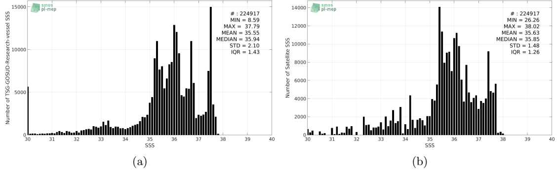
Figure 2: Histograms of SSS from TSG-GOSUD-Research-vessel (a) and SMOS-L4-CATDS-CECOS-IFREMER-V2-WEEKLY-0.5DEG (b) considering all match-up pairs per bins of 0.1 over the Amazon and Orinoco river plumes Pi-MEP region and for the full satellite product period.
