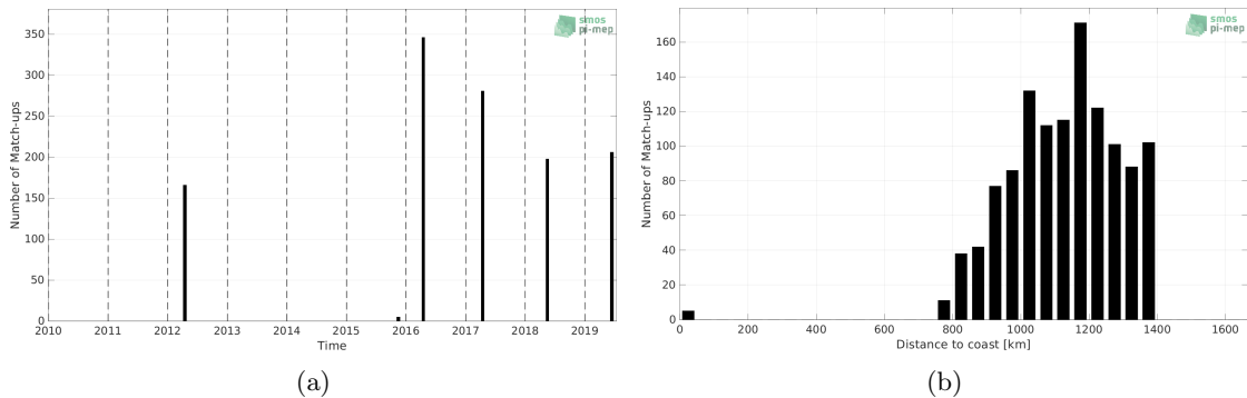
Figure 1: Number of match-ups between TSG (Polarstern) and SMOS SSS L4 v2 - Daily (BEC) SSS as a function of time (a) and as function of the distance to coast (b) over the Amazon and Orinoco river plumes Pi-MEP region and for the full satellite product period.
