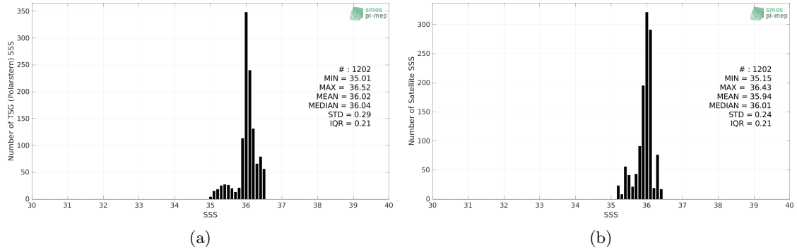
Figure 2: Histograms of SSS from TSG (Polarstern) (a) and SMOS SSS L4 v2 - Daily (BEC) (b) considering all match-up pairs per bins of 0.1 over the Amazon and Orinoco river plumes Pi-MEP region and for the full satellite product period.
