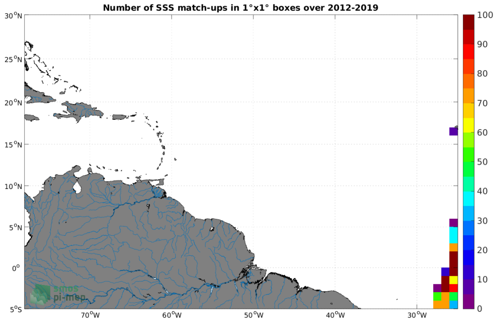
Figure 4: Number of SSS match-ups between TSG (Polarstern) SSS and the SMOS SSS L4 v2 - Daily (BEC) SSS product for the Amazon and Orinoco river plumes Pi-MEP region over 1^\circ \times 1^\circ boxes and for the full satellite product period.
