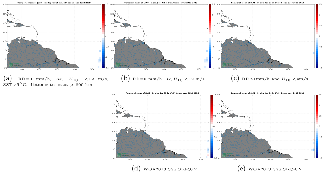
Figure 12: Temporal mean gridded over spatial boxes of size 1^\circ \times 1^\circ of \Delta SSS (SMOS SSS L4 v2 - Daily (BEC) - TSG (Polarstern)) for 5 different subdatasets corresponding to:RR=0 mm/h, 3 < U_{10} < 12 m/s, SST >5^\circ\text{C} , distance to coast > 800 km (a), RR=0 mm/h, 3 < U_{10} < 12 m/s (b), RR >1 mm/h and U_{10} < 4 m/s (c), WOA2013 SSS Std <0.2 (d), WOA2013 SSS Std >0.2 (e).
