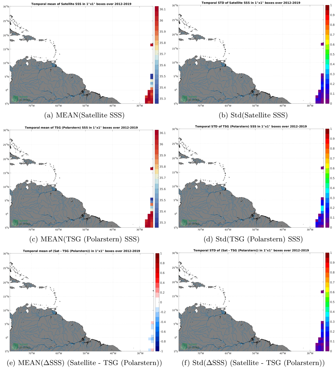
Figure 6: Temporal mean (left) and Std (right) of SSS from SMOS SSS L4 v2 - Daily (BEC) (top), TSG (Polarstern) (middle), and of \Delta SSS (Satellite - TSG (Polarstern)). Only match-up pairs are used to generate these maps.
