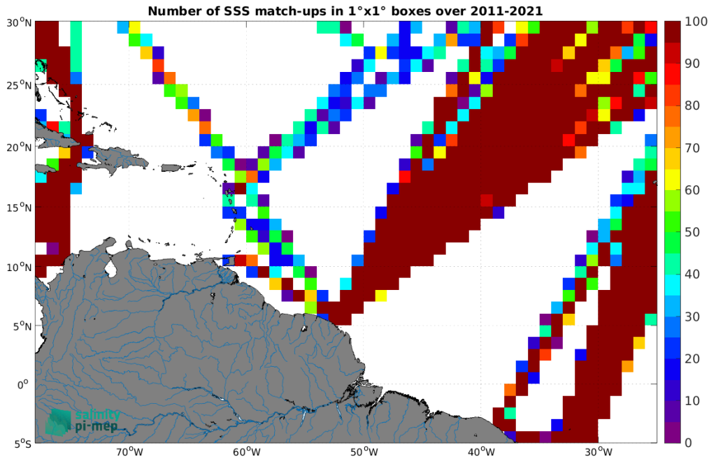
Figure 5: Number of SSS match-ups between TSG (LEGOS-DM) SSS and the SMOS SSS L4 v2 - Daily (BEC) SSS product for the Amazon and Orinoco river plumes Pi-MEP region over 1^\circ \times 1^\circ boxes and for the full satellite product period.
