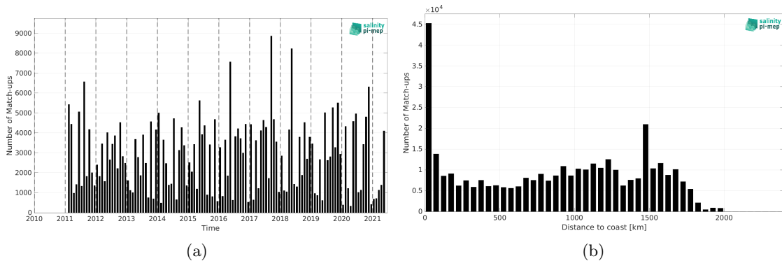
Figure 2: Number of match-ups between TSG (LEGOS-DM) and SMOS SSS L4 v2 - Daily (BEC) SSS as a function of time (a) and as function of the distance to coast (b) over the Amazon and Orinoco river plumes Pi-MEP region and for the full satellite product period.
