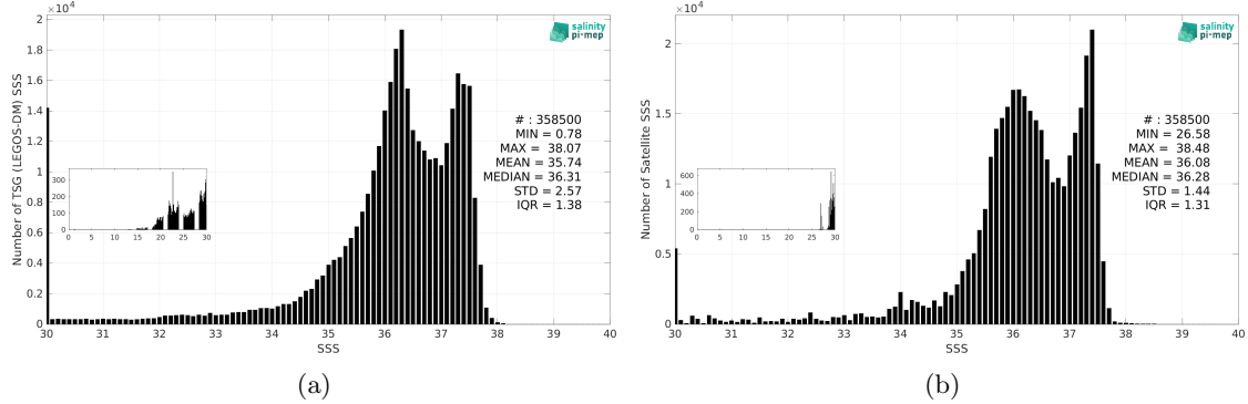
Figure 3: Histograms of SSS from TSG (LEGOS-DM) (a) and SMOS SSS L4 v2 - Daily (BEC) (b) considering all match-up pairs per bins of 0.1 over the Amazon and Orinoco river plumes Pi-MEP region and for the full satellite product period.
