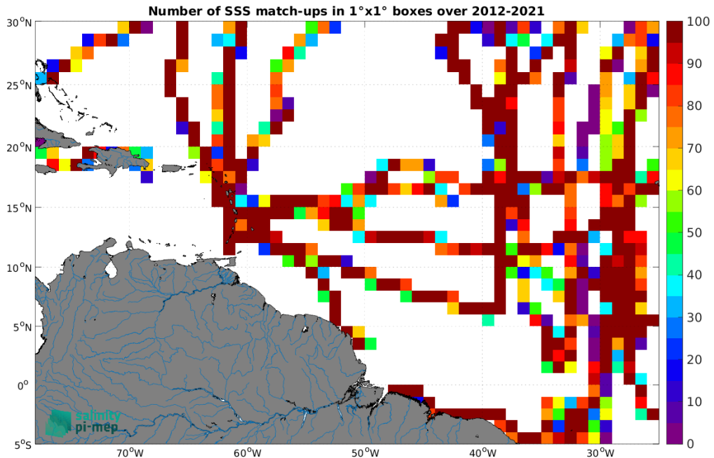
Figure 5: Number of SSS match-ups between TSG (GOSUD-Sailing-ship) SSS and the SMOS SSS L4 v2 - Daily (BEC) SSS product for the Amazon and Orinoco river plumes Pi-MEP region over 1°×1° boxes and for the full satellite product period.
