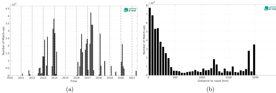
Figure 1: Number of match-ups between TSG (GOSUD-Research-vessel) and SMOS SSS L4 v2 - Daily (BEC) SSS as a function of time (a) and as function of the distance to coast (b) over the Amazon and Orinoco river plumes Pi-MEP region and for the full satellite product period.
