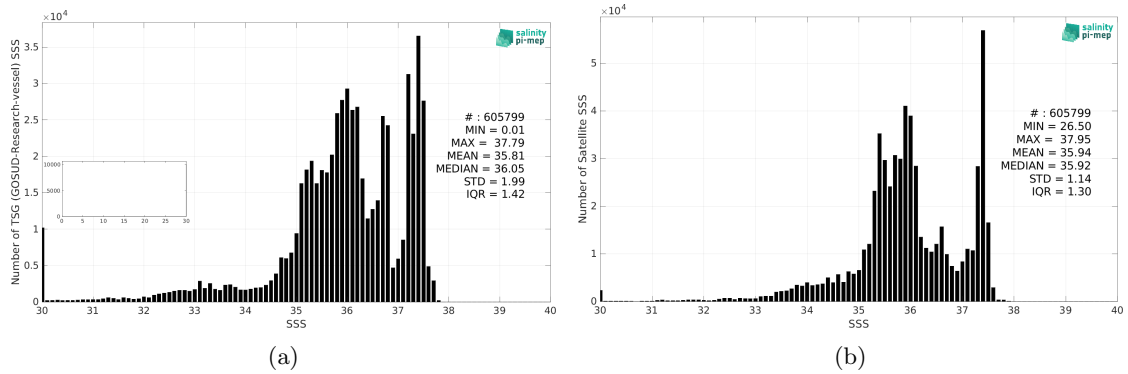
Figure 2: Histograms of SSS from TSG (GOSUD-Research-vessel) (a) and SMOS SSS L4 v2 - Daily (BEC) (b) considering all match-up pairs per bins of 0.1 over the Amazon and Orinoco river plumes Pi-MEP region and for the full satellite product period.
