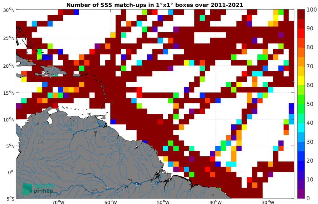
Figure 4: Number of SSS match-ups between TSG (GOSUD-Research-vessel) SSS and the SMOS SSS L4 v2 - Daily (BEC) SSS product for the Amazon and Orinoco river plumes Pi-MEP region over 1^\circ \times 1^\circ boxes and for the full satellite product period.
