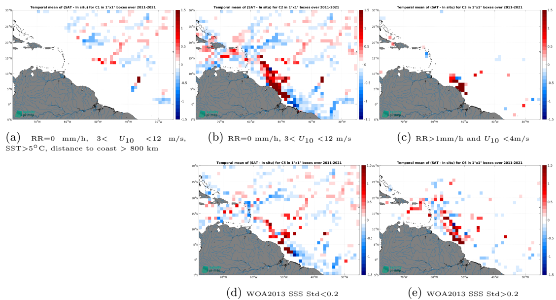
Figure 12: Temporal mean gridded over spatial boxes of size 1^\circ \times 1^\circ of \Delta\text{SSS} (SMOS SSS L4 v2 - Daily (BEC) - TSG (GOSUD-Research-vessel)) for 5 different subdatasets corresponding to:RR=0 mm/h, 3 < U_{10} < 12 m/s, SST >5^\circ\text{C} , distance to coast > 800 km (a), RR=0 mm/h, 3 < U_{10} < 12 m/s (b), RR >1 mm/h and U_{10} < 4 m/s (c), WOA2013 SSS Std <0.2 (d), WOA2013 SSS Std >0.2 (e).
