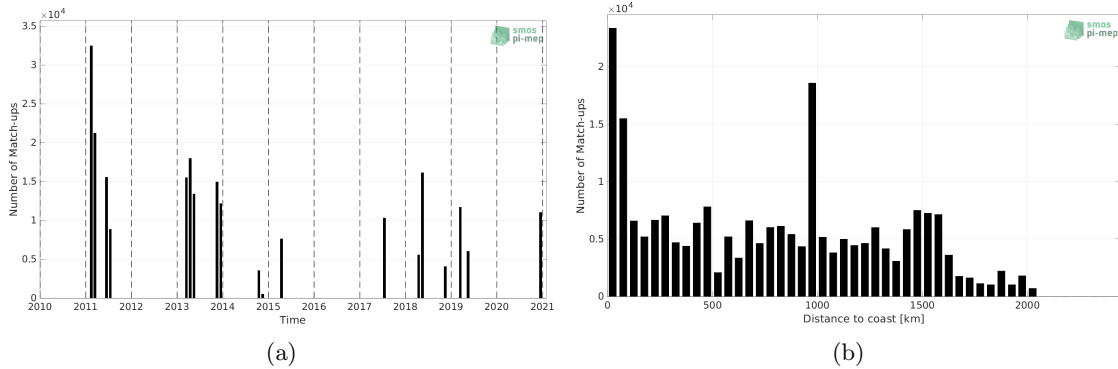
Figure 1: Number of match-ups between TSG (CSIC-UTM) and SMOS SSS L4 v2 - Daily (BEC) SSS as a function of time (a) and as function of the distance to coast (b) over the Amazon and Orinoco river plumes Pi-MEP region and for the full satellite product period.
