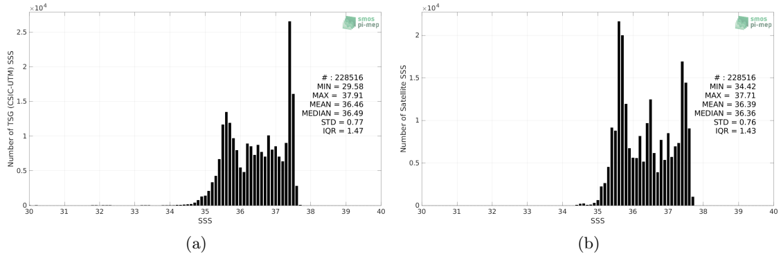
Figure 2: Histograms of SSS from TSG (CSIC-UTM) (a) and SMOS SSS L4 v2 - Daily (BEC) (b) considering all match-up pairs per bins of 0.1 over the Amazon and Orinoco river plumes Pi-MEP region and for the full satellite product period.
