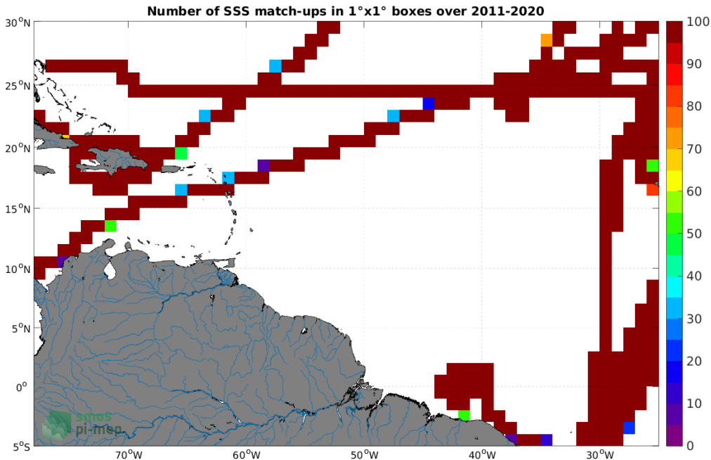
Figure 4: Number of SSS match-ups between TSG (CSIC-UTM) SSS and the SMOS SSS L4 v2 - Daily (BEC) SSS product for the Amazon and Orinoco river plumes Pi-MEP region over 1^{\circ} \times 1^{\circ} boxes and for the full satellite product period.
