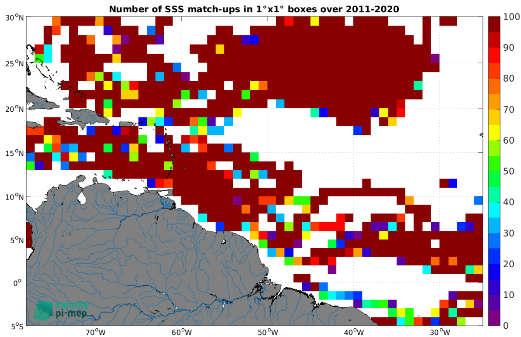
Figure 4: Number of SSS match-ups between Surface drifters SSS and the SMOS SSS L4 v2 - Daily (BEC) SSS product for the Amazon and Orinoco river plumes Pi-MEP region over 1^\circ \times 1^\circ boxes and for the full satellite product period.
