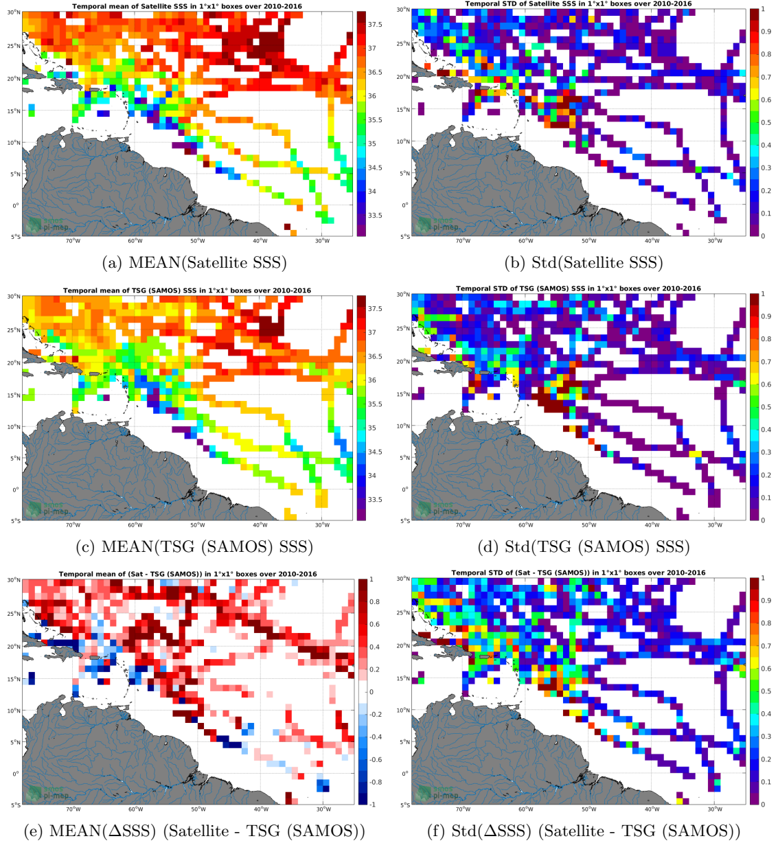
Figure 6: Temporal mean (left) and Std (right) of SSS from SMOS SSS L3 v3 Monthly (ICDC) (top), TSG (SAMOS) (middle), and of \Delta SSS (Satellite - TSG (SAMOS)). Only match-up pairs are used to generate these maps.
