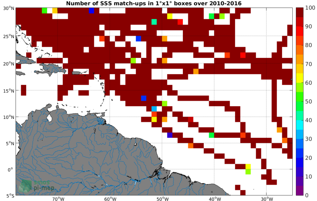
Figure 4: Number of SSS match-ups between TSG (SAMOS) SSS and the SMOS SSS L3 v3 Monthly (ICDC) SSS product for the Amazon and Orinoco river plumes Pi-MEP region over 1^\circ \times 1^\circ boxes and for the full satellite product period.
