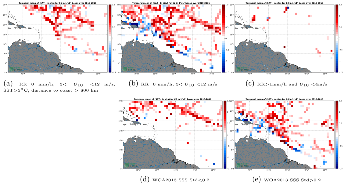
Figure 12: Temporal mean gridded over spatial boxes of size 1^\circ \times 1^\circ of \Delta SSS (SMOS SSS L3 v3 Monthly (ICDC) - TSG (SAMOS)) for 5 different subdatasets corresponding to: RR=0 mm/h, 3 < U_{10} < 12 m/s, SST > 5^\circ C , distance to coast > 800 km (a), RR=0 mm/h, 3 < U_{10} < 12 m/s (b), RR > 1 mm/h and U_{10} < 4 m/s (c), WOA2013 SSS Std < 0.2 (d), WOA2013 SSS Std > 0.2 (e).
