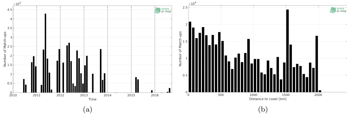
Figure 1: Number of match-ups between TSG (SAMOS) and SMOS SSS L3 v3 Monthly (ICDC) SSS as a function of time (a) and as function of the distance to coast (b) over the Amazon and Orinoco river plumes Pi-MEP region and for the full satellite product period.
