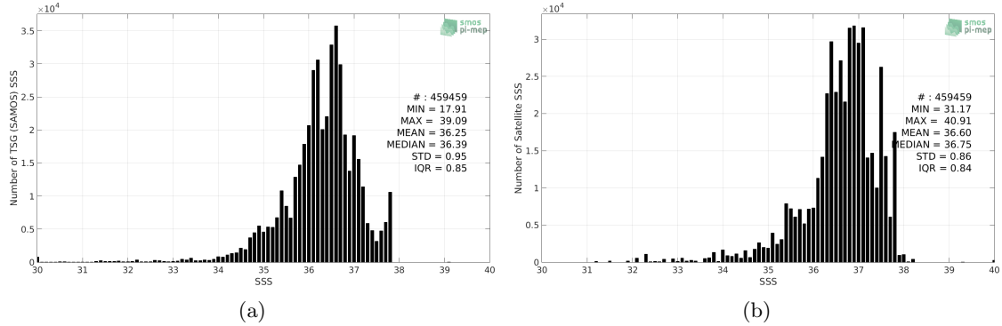
Figure 2: Histograms of SSS from TSG (SAMOS) (a) and SMOS SSS L3 v3 Monthly (ICDC) (b) considering all match-up pairs per bins of 0.1 over the Amazon and Orinoco river plumes Pi-MEP region and for the full satellite product period.
