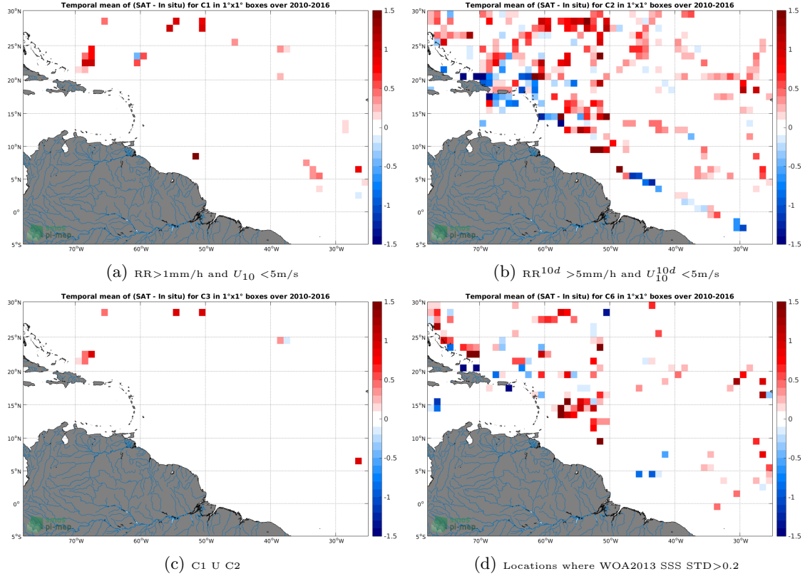
Figure 12: Temporal mean gridded over spatial boxes of size 1^\circ \times 1^\circ of \Delta SSS (SMOS-L3-ICDC-V3-MONTHLY-0.5DEG - TSG-SAMOS) for 4 different subdatasets corresponding to: RR > 1\text{mm/h} and U_{10} < 5\text{m/s} (a), RR^{10d} > 5\text{mm/h} and U_{10}^{10d} < 5\text{m/s} (b), C1 U C2 (c), Locations where WOA2013 SSS STD > 0.2 (d).
