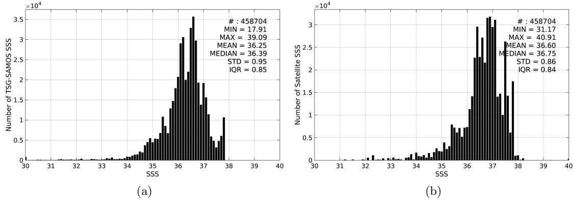
Figure 2: Histograms of SSS from TSG-SAMOS (a) and SMOS-L3-ICDC-V3-MONTHLY-0.5DEG (b) considering all match-up pairs per bins of 0.1 over the Amazon and Orinoco river plumes Pi-MEP region and for the full satellite product period.
