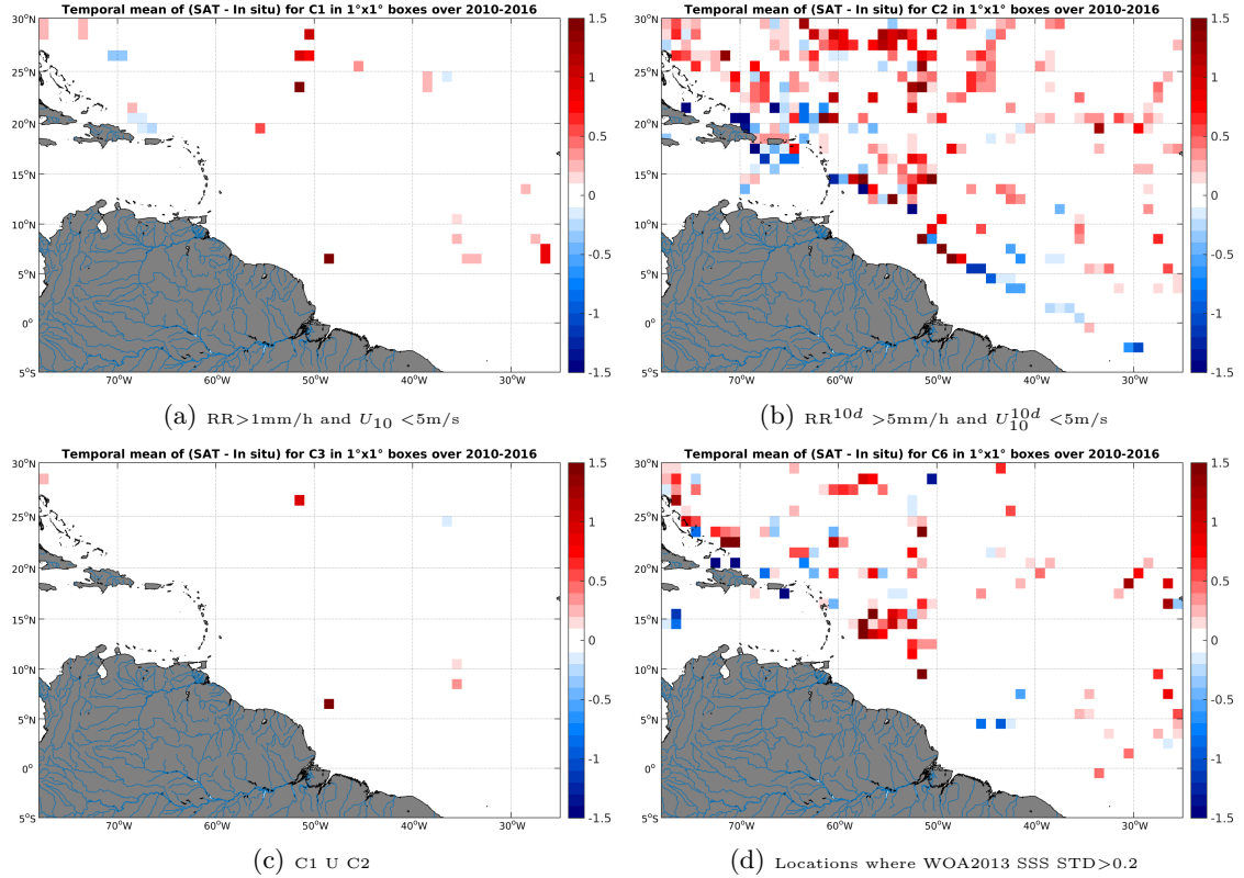
Figure 12: Temporal mean gridded over spatial boxes of size 1^\circ \times 1^\circ of \Delta SSS (SMOS-L3-ICDC-V3-MONTHLY-0.5DEG - TSG-SAMOS) for 4 different subdatasets corresponding to: RR > 1mm/h and U_{10} < 5\text{m/s} (a), RR^{10d} > 5\text{mm/h} and U_{10}^{10d} < 5\text{m/s} (b), C1 U C2 (c), Locations where WOA2013 SSS STD > 0.2 (d).
