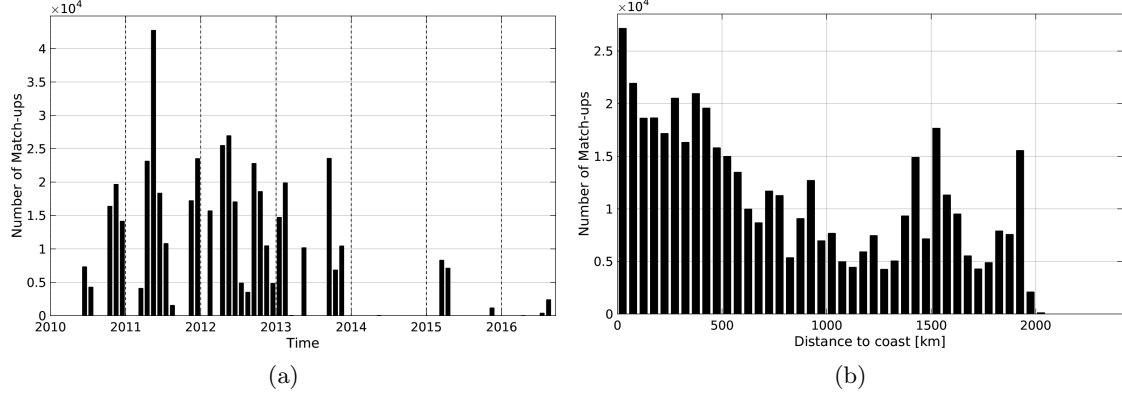
Figure 1: Number of match-ups between TSG-SAMOS and SMOS-L3-ICDC-V3-MONTHLY-0.5DEG SSS as a function of time (a) and as function of the distance to coast (b) over the Amazon and Orinoco river plumes Pi-MEP region and for the full satellite product period.
