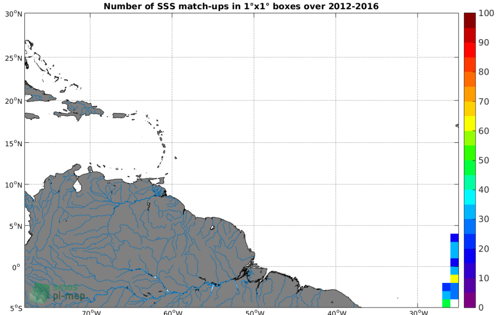
Figure 4: Number of SSS match-ups between TSG-POLARSTERN SSS and the SMOS-L3-ICDC-V3-MONTHLY-0.5DEG SSS product for the Amazon and Orinoco river plumes Pi-MEP region over 1°x1° boxes and for the full satellite product period.
