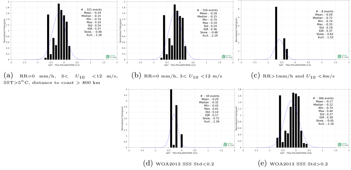
Figure 13: Normalized histogram of \Delta SSS (SMOS-L3-ICDC-V3-MONTHLY-0.5DEG - TSG-POLARSTERN) for 5 different subdatasets corresponding to: RR=0 mm/h, 3 < U_{10} < 12 m/s, SST>5°C, distance to coast > 800 km (a), RR=0 mm/h, 3 < U_{10} < 12 m/s (b), RR>1 mm/h and U_{10} < 4 m/s (c), WOA2013 SSS Std<0.2 (d), WOA2013 SSS Std>0.2 (e).
