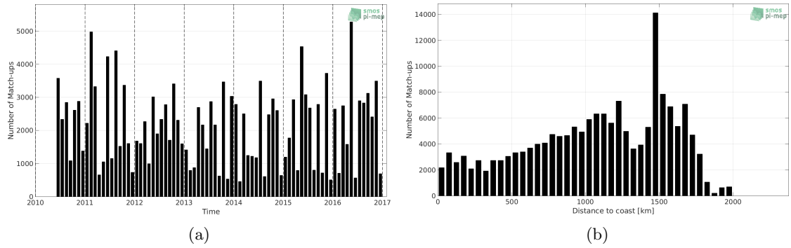
Figure 1: Number of match-ups between TSG (LEGOS-DM) and SMOS SSS L3 v3 Monthly (ICDC) SSS as a function of time (a) and as function of the distance to coast (b) over the Amazon and Orinoco river plumes Pi-MEP region and for the full satellite product period.
