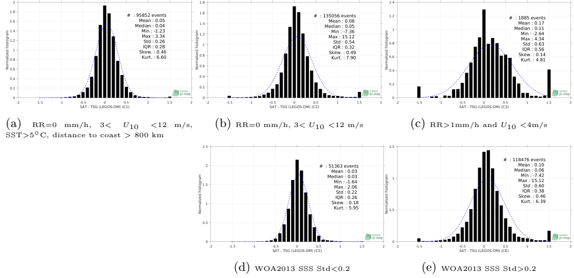
Figure 13: Normalized histogram of \Delta SSS (SMOS SSS L3 v3 Monthly (ICDC) - TSG (LEGOS-DM)) for 5 different subdatasets corresponding to: RR=0 mm/h, 3 < U_{10} < 12 m/s, SST>5°C, distance to coast > 800 km (a), RR=0 mm/h, 3 < U_{10} < 12 m/s (b), RR>1mm/h and U_{10} < 4 m/s (c), WOA2013 SSS Std<0.2 (d), WOA2013 SSS Std>0.2 (e).
