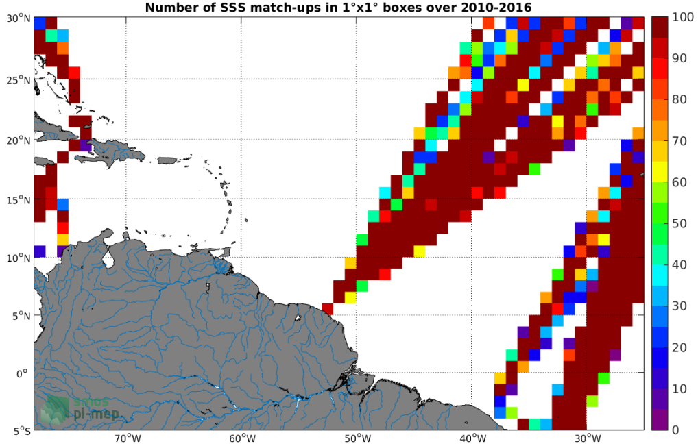
Figure 4: Number of SSS match-ups between TSG (LEGOS-DM) SSS and the SMOS SSS L3 v3 Monthly (ICDC) SSS product for the Amazon and Orinoco river plumes Pi-MEP region over 1^\circ \times 1^\circ boxes and for the full satellite product period.
