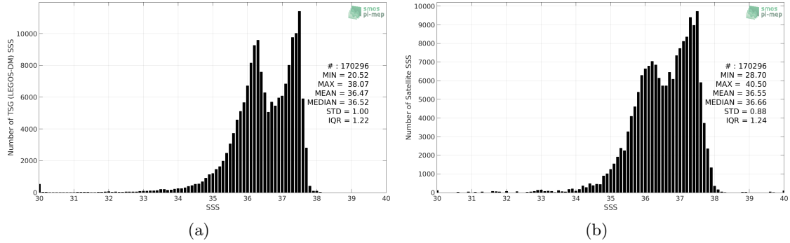
Figure 2: Histograms of SSS from TSG (LEGOS-DM) (a) and SMOS SSS L3 v3 Monthly (ICDC) (b) considering all match-up pairs per bins of 0.1 over the Amazon and Orinoco river plumes Pi-MEP region and for the full satellite product period.
