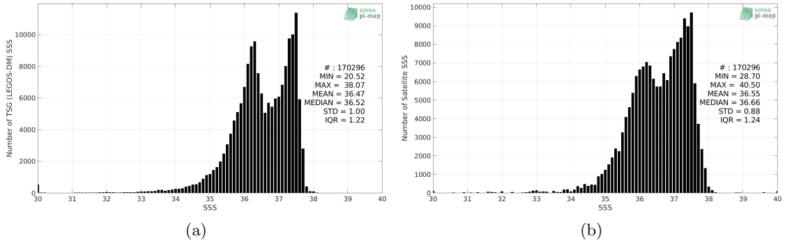
Figure 2: Histograms of SSS from TSG (LEGOS-DM) (a) and SMOS SSS L3 v3 Monthly (ICDC) (b) considering all match-up pairs per bins of 0.1 over the Amazon and Orinoco river plumes Pi-MEP region and for the full satellite product period.
