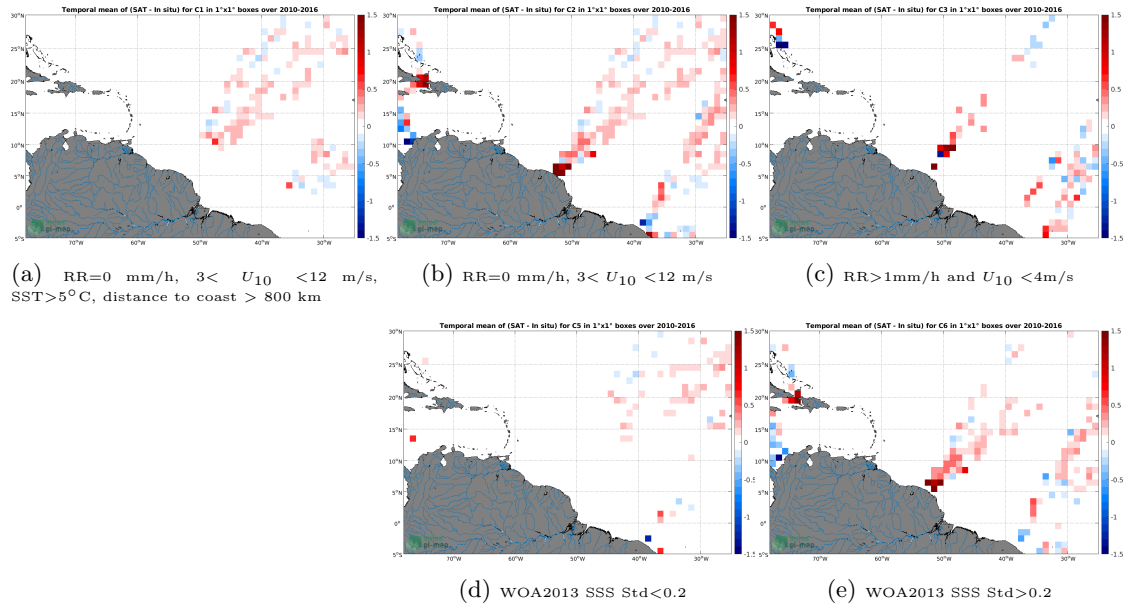
Figure 12: Temporal mean gridded over spatial boxes of size 1^\circ \times 1^\circ of \Delta SSS (SMOS SSS L3 v3 Monthly (ICDC) - TSG (LEGOS-DM)) for 5 different subdatasets corresponding to:RR=0 mm/h, 3 < U_{10} < 12 m/s, SST >5^\circ\text{C} , distance to coast > 800 km (a), RR=0 mm/h, 3 < U_{10} < 12 m/s (b), RR >1 mm/h and U_{10} < 4 m/s (c), WOA2013 SSS Std <0.2 (d), WOA2013 SSS Std >0.2 (e).
