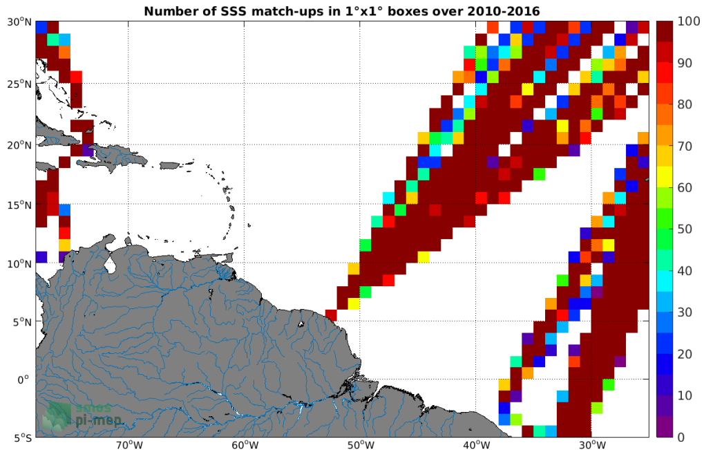
Figure 4: Number of SSS match-ups between TSG (LEGOS-DM) SSS and the SMOS SSS L3 v3 Monthly (ICDC) SSS product for the Amazon and Orinoco river plumes Pi-MEP region over 1°x1° boxes and for the full satellite product period.
