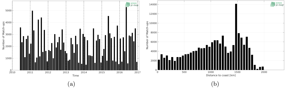
Figure 1: Number of match-ups between TSG-LEGOS-DM and SMOS-L3-ICDC-V3-MONTHLY-0.5DEG SSS as a function of time (a) and as function of the distance to coast (b) over the Amazon and Orinoco river plumes Pi-MEP region and for the full satellite product period.
