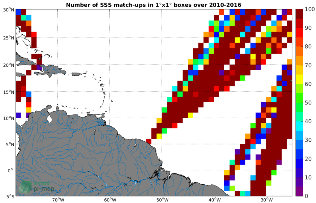
Figure 4: Number of SSS match-ups between TSG-LEGOS-DM SSS and the SMOS-L3-ICDC-V3-MONTHLY-0.5DEG SSS product for the Amazon and Orinoco river plumes Pi-MEP region over 1^\circ \times 1^\circ boxes and for the full satellite product period.
