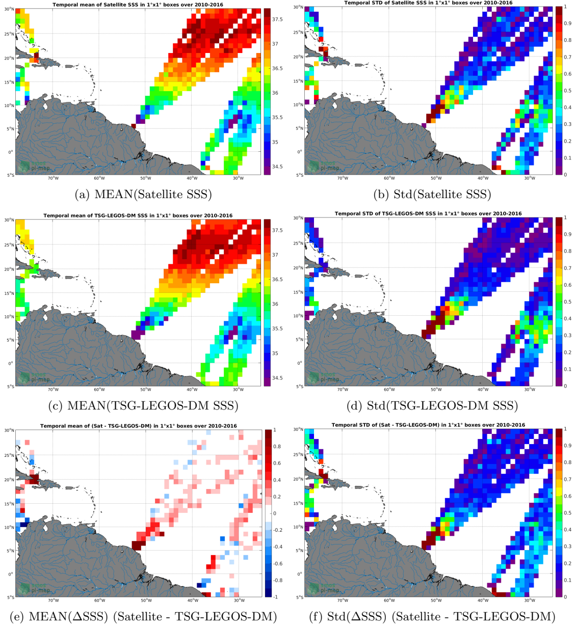
Figure 6: Temporal mean (left) and Std (right) of SSS from SMOS-L3-ICDC-V3-MONTHLY-0.5DEG (top), TSG-LEGOS-DM (middle), and of \Delta SSS (Satellite - TSG-LEGOS-DM). Only match-up pairs are used to generate these maps.
