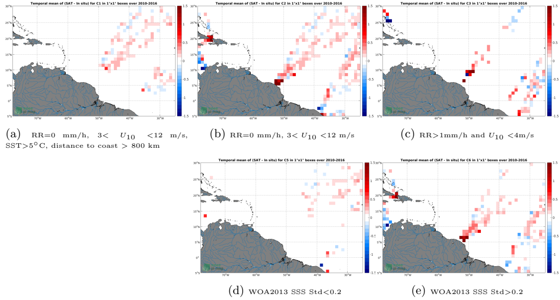
Figure 12: Temporal mean gridded over spatial boxes of size 1^\circ \times 1^\circ of \Delta SSS (SMOS-L3-ICDC-V3-MONTHLY-0.5DEG - TSG-LEGOS-DM) for 5 different subdatasets corresponding to: RR=0 mm/h, 3 < U_{10} < 12 m/s, SST > 5^\circ C , distance to coast > 800 km (a), RR=0 mm/h, 3 < U_{10} < 12 m/s (b), RR > 1 mm/h and U_{10} < 4 m/s (c), WOA2013 SSS Std < 0.2 (d), WOA2013 SSS Std > 0.2 (e).
