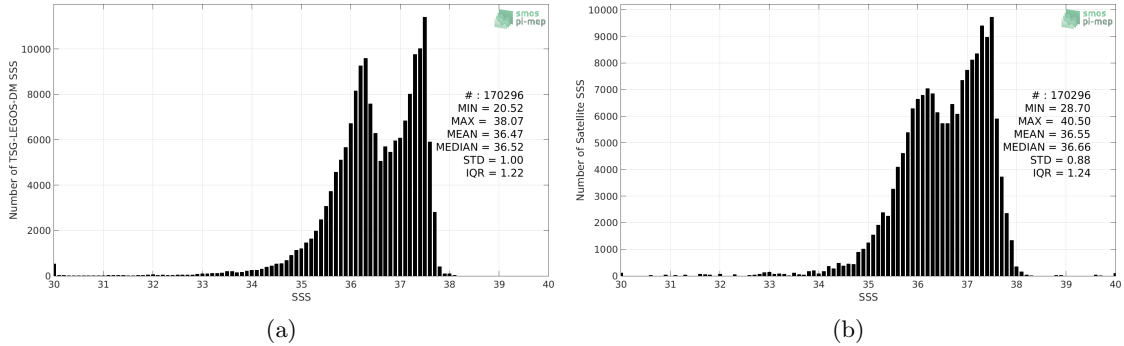
Figure 2: Histograms of SSS from TSG-LEGOS-DM (a) and SMOS-L3-ICDC-V3-MONTHLY-0.5DEG (b) considering all match-up pairs per bins of 0.1 over the Amazon and Orinoco river plumes Pi-MEP region and for the full satellite product period.
