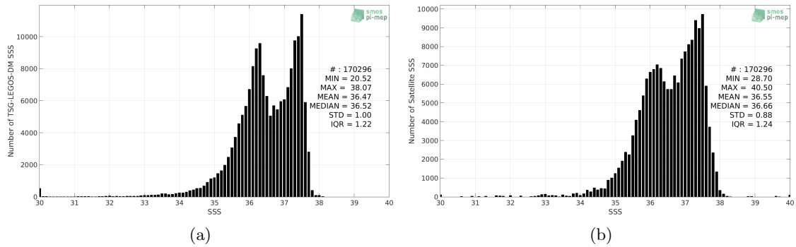
Figure 2: Histograms of SSS from TSG-LEGOS-DM (a) and SMOS-L3-ICDC-V3-MONTHLY-0.5DEG (b) considering all match-up pairs per bins of 0.1 over the Amazon and Orinoco river plumes Pi-MEP region and for the full satellite product period.
