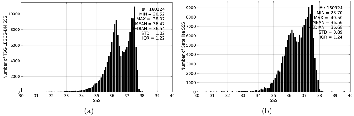
Figure 2: Histograms of SSS from TSG-LEGOS-DM (a) and SMOS-L3-ICDC-V3-MONTHLY-0.5DEG (b) considering all match-up pairs per bins of 0.1 over the Amazon and Orinoco river plumes Pi-MEP region and for the full satellite product period.
