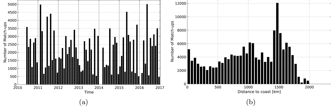
Figure 1: Number of match-ups between TSG-LEGOS-DM and SMOS-L3-ICDC-V3-MONTHLY-0.5DEG SSS as a function of time (a) and as function of the distance to coast (b) over the Amazon and Orinoco river plumes Pi-MEP region and for the full satellite product period.
