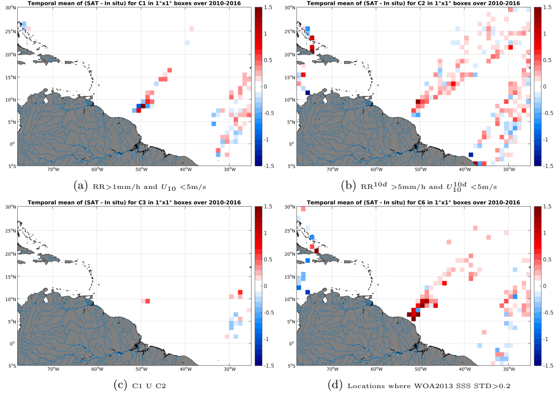
Figure 12: Temporal mean gridded over spatial boxes of size 1^\circ \times 1^\circ of \Delta SSS (SMOS-L3-ICDC-V3-MONTHLY-0.5DEG - TSG-LEGOS-DM) for 4 different subdatasets corresponding to: RR > 1 mm/h and U_{10} < 5 m/s (a), RR^{10d} > 5 mm/h and U_{10}^{10d} < 5 m/s (b), C1 U C2 (c), Locations where WOA2013 SSS STD > 0.2 (d).
