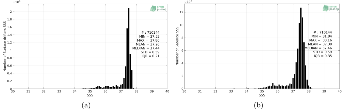
Figure 2: Histograms of SSS from Surface drifters (a) and SMOS SSS L3 v3 Monthly (ICDC) (b) considering all match-up pairs per bins of 0.1 over the Amazon and Orinoco river plumes Pi-MEP region and for the full satellite product period.
