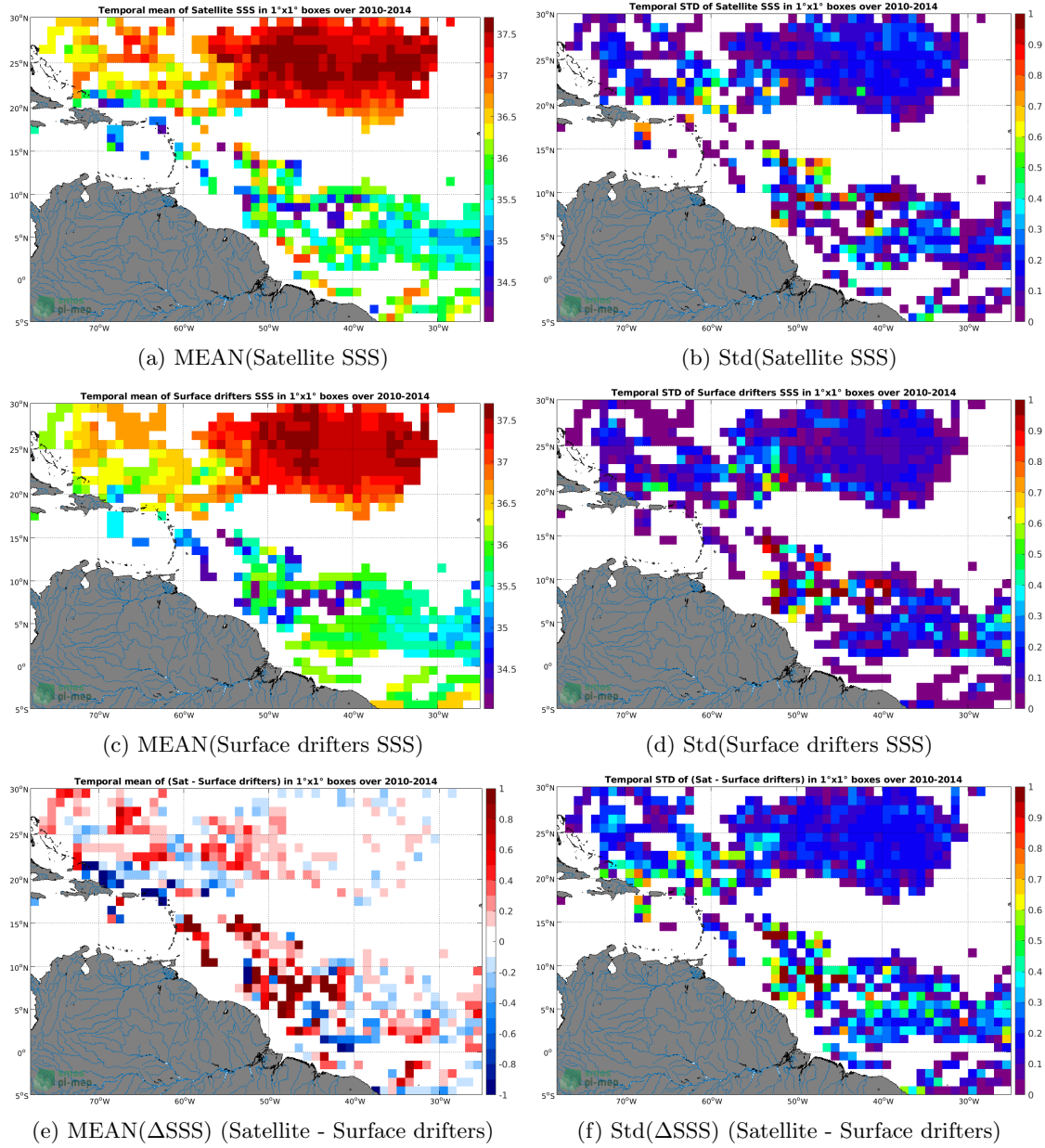
Figure 5: Temporal mean (left) and Std (right) of SSS from SMOS SSS L3 v3 Monthly (ICDC) (top), Surface drifters (middle), and of \Delta SSS (Satellite - Surface drifters). Only match-up pairs are used to generate these maps.
