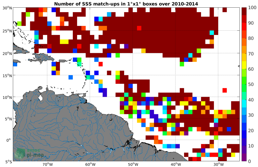
Figure 3: Number of SSS match-ups between Surface drifters SSS and the SMOS SSS L3 v3 Monthly (ICDC) SSS product for the Amazon and Orinoco river plumes Pi-MEP region over 1^\circ \times 1^\circ boxes and for the full satellite product period.
