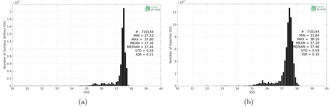
Figure 2: Histograms of SSS from Surface drifters (a) and SMOS SSS L3 v3 Monthly (ICDC) (b) considering all match-up pairs per bins of 0.1 over the Amazon and Orinoco river plumes Pi-MEP region and for the full satellite product period.
