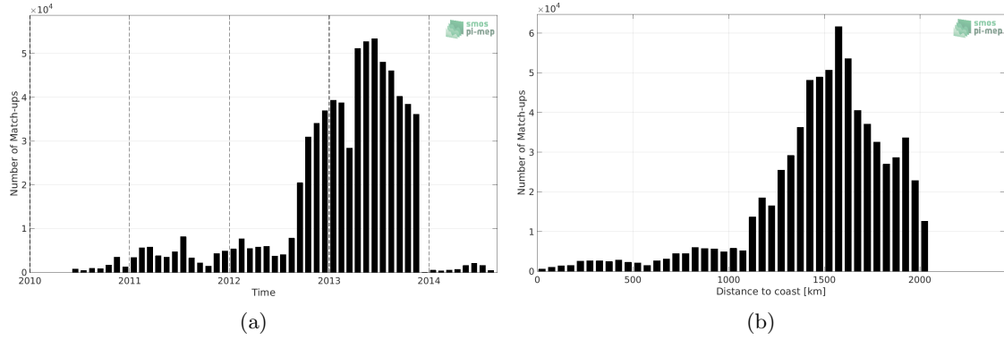
Figure 1: Number of match-ups between Surface drifters and SMOS SSS L3 v3 Monthly (ICDC) SSS as a function of time (a) and as function of the distance to coast (b) over the Amazon and Orinoco river plumes Pi-MEP region and for the full satellite product period.
