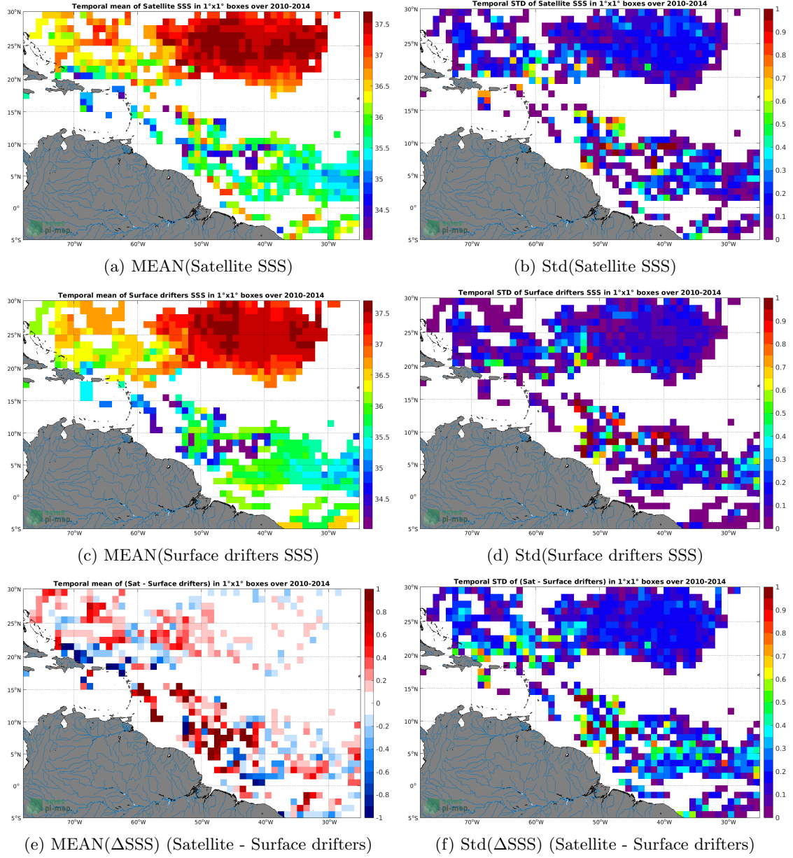
Figure 5: Temporal mean (left) and Std (right) of SSS from SMOS SSS L3 v3 Monthly (ICDC') (top), Surface drifters (middle), and of \Delta SSS (Satellite - Surface drifters). Only match-up pairs are used to generate these maps.
