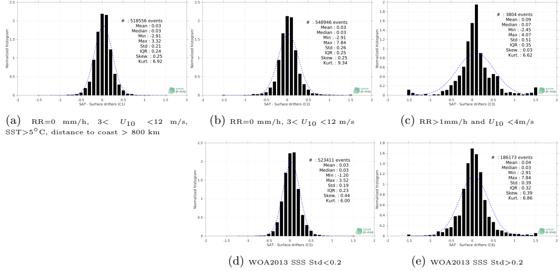
Figure 12: Normalized histogram of \Delta SSS (SMOS SSS L3 v3 Monthly (ICDC) - Surface drifters) for 5 different subdatasets corresponding to: RR=0 mm/h, 3 < U_{10} < 12 m/s, SST>5°C, distance to coast > 800 km (a), RR=0 mm/h, 3 < U_{10} < 12 m/s (b), RR>1mm/h and U_{10} < 4 m/s (c), WOA2013 SSS Std<0.2 (d), WOA2013 SSS Std>0.2 (e).
