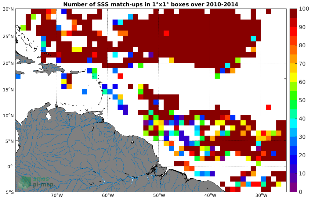
Figure 3: Number of SSS match-ups between Surface drifters SSS and the SMOS SSS L3 v3 Monthly (ICDC) SSS product for the Amazon and Orinoco river plumes Pi-MEP region over 1°x1° boxes and for the full satellite product period.
