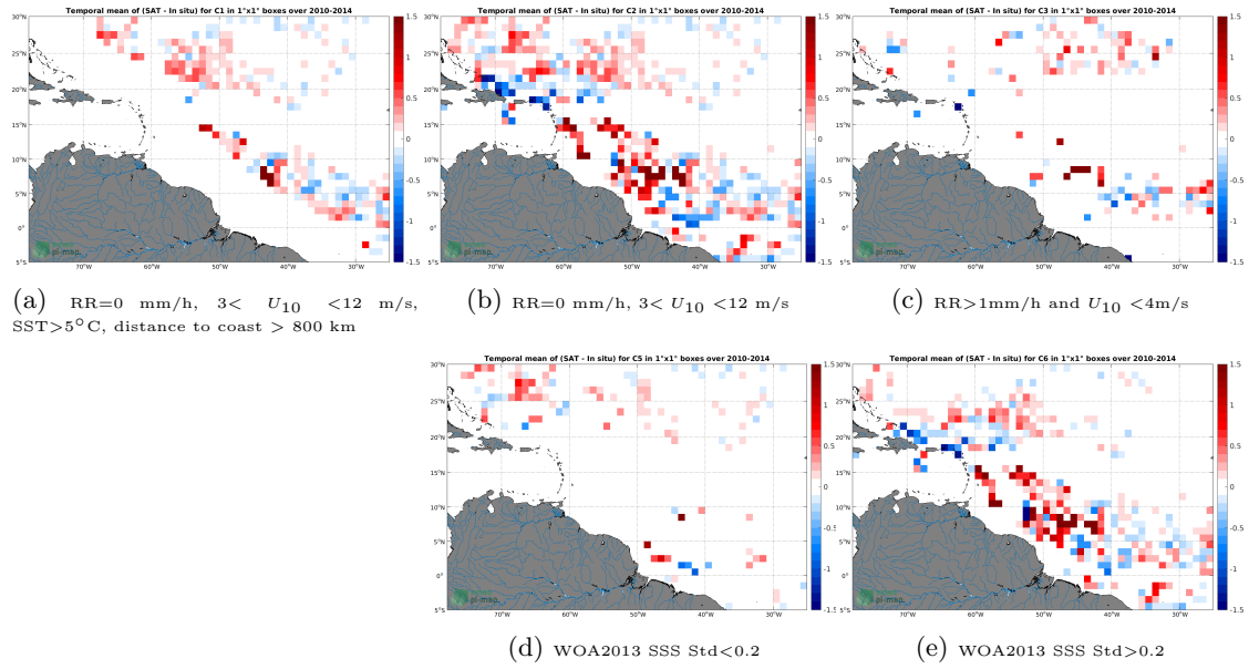
Figure 11: Temporal mean gridded over spatial boxes of size 1^\circ \times 1^\circ of \Delta SSS (SMOS SSS L3 v3 Monthly (ICDC) - Surface drifters) for 5 different subdatasets corresponding to: RR=0 mm/h, 3 < U_{10} < 12 m/s, SST > 5^\circ C , distance to coast > 800 km (a), RR=0 mm/h, 3 < U_{10} < 12 m/s (b), RR > 1 mm/h and U_{10} < 4 m/s (c), WOA2013 SSS Std < 0.2 (d), WOA2013 SSS Std > 0.2 (e).
