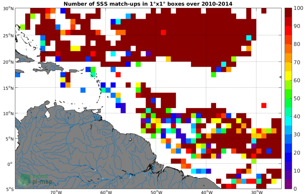
Figure 3: Number of SSS match-ups between Surface drifters SSS and the SMOS-L3-ICDC-V3-MONTHLY-0.5DEG SSS product for the Amazon and Orinoco river plumes Pi-MEP region over 1^\circ \times 1^\circ boxes and for the full satellite product period.
