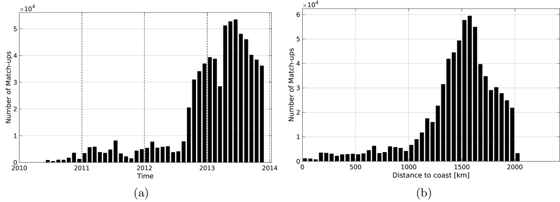
Figure 1: Number of match-ups between Surface drifters and SMOS-L3-ICDC-V3-MONTHLY-0.5DEG SSS as a function of time (a) and as function of the distance to coast (b) over the Amazon and Orinoco river plumes Pi-MEP region and for the full satellite product period.
