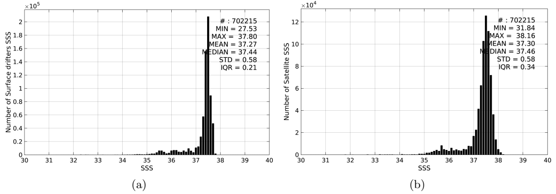
Figure 2: Histograms of SSS from Surface drifters (a) and SMOS-L3-ICDC-V3-MONTHLY-0.5DEG (b) considering all match-up pairs per bins of 0.1 over the Amazon and Orinoco river plumes Pi-MEP region and for the full satellite product period.
